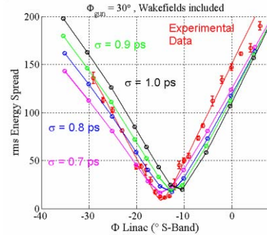
Figure 7: rms Energy spread vs booster Phase for various initial rms bunch length; wakefields are included
