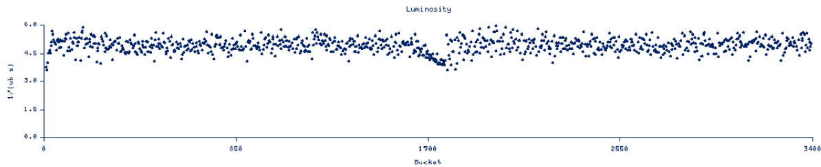
Figure 3: Special by-3 pattern with short trains of 5 bunches out of 6 (till bucket 585), and then every 4 th train the middle of the 5 bunches is removed. A straight by-3 part is around bucket 1700±70. The top shows the LER bunch current after coasting for 45 min, next is the HER current with no change and the luminosity. The bottom shows the initial luminosity, when the currents were flat, indicating a drop induced by the electron cloud.
