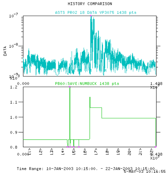
Figure 2: Pressure activity (top, in Torr) and number of bunches (bottom) when going from by-4 to a by-3 pattern.
