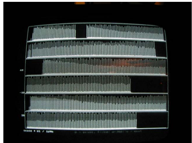
Figure 6: By-2 pattern with short “trains” (2,4,2,4...) shows only a luminosity loss for the second bunch.
