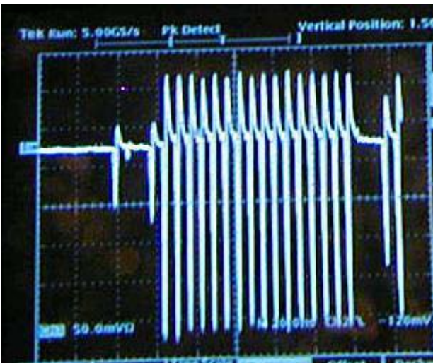
Figure 4: BPM intensity signals of first few bunches in LER (top) and HER (bottom), (20ns/div).
