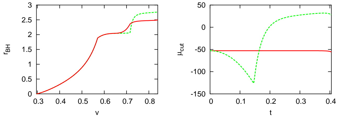
FIG. 4: The size of the apparent horizon (left) and the reduced mass \mu at the cut-off (right) for the same initial conditions as in Fig. 3. Solid and dashed lines show the values corresponding to Dirichlet and Neumann boundary conditions at the cut-off.
