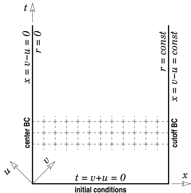
FIG. 1: Coordinate choice.
