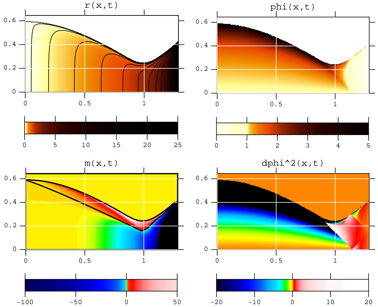
FIG. 3: Global structure of the spacetime resulting from the evolution of the truncated 1/r^2 field profile (26) for the values of parameters A = 16 , R_0 = 4 . Thick black lines on m(x, t) plot show the locations of the apparent horizon and the singularity.
