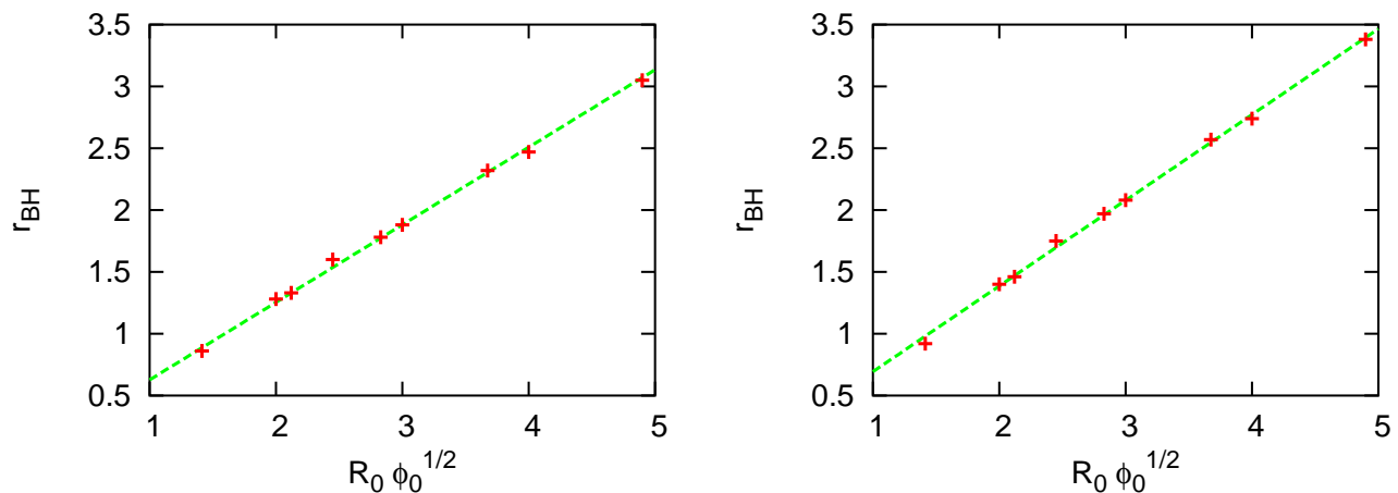
FIG. 5: The size of the black hole formed in the collapse of the truncated 1/r^2 field profile (26) as a function of parameters, shown for Dirichlet (left) and Neumann (right) boundary conditions at the cut-off.
