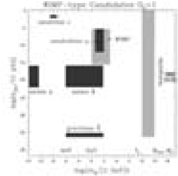
Fig. 1. Cross sections and masses of WIMP dark matter candidates. Black hole remnant (BHR) is included.
