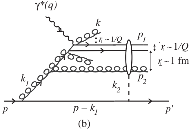
FIG. 5: Low-order rescattering correction to DIS in the parton model frame where the virtual photon momentum is along the negative z -axis with q = (q^+, q^-, \mathbf{q}_\perp) \simeq (-m_p x_B, 2\nu, \mathbf{0}) and the target is at rest, p = (m_p, m_p, \mathbf{0}) . The struck parton absorbs nearly all the photon momentum, p_1 \simeq (0, 2\nu, \mathbf{p}_{1\perp}) (aligned jet configuration). In (a) the virtual photon strikes a quark and the diffractive system is formed by the q\bar{q} pair ( p_1, p_2 ) which rescatters coherently from the target via ‘instantaneous’ longitudinal ( A^+ ) gluon exchange with momentum k_2 . In (b) the Q\bar{Q} quark pair which is produced in the \gamma^*g \rightarrow Q\bar{Q} subprocess has a small transverse size r_\perp \sim 1/Q and rescatters like a gluon. The diffractive system is then formed by the (Q\bar{Q})g system. The possibility of hard gluon emission close to the photon vertex is indicated. Such radiation (labeled k ) emerges at a short transverse distance from the struck parton and is not resolved in the rescattering.
