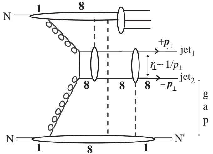
FIG. 7: Illustration of diffraction through rescattering in NN \rightarrow 2 \text{ jets} + X in analogy with, and using the same notation as, the DIS case in Fig. 5. The compact q\bar{q} pair which forms the jets is assumed to be in a color octet ( \mathbf{8} ) configuration. This pair rescatters coherently and thus retains its color.
