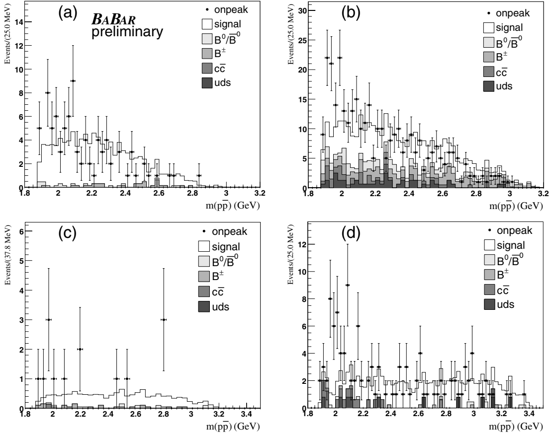
Figure 9: Invariant mass distributions for p\bar{p} pairs in the signal sample for (a) for B^0 \rightarrow D^{*-}p\bar{p}\pi^+ ; (b) for B^0 \rightarrow D^-p\bar{p}\pi^+ ; (c) for B^0 \rightarrow \bar{D}^{*0}p\bar{p} ; and (d) for B^0 \rightarrow \bar{D}^0p\bar{p} , respectively. The cross-hatched histograms describe the contributions from different background processes. The open histogram is the expected contribution from the phase space signal MC simulation.
