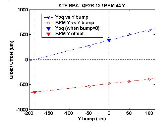
Figure 3: Beam-quad offset (“Ybq”), derived from changes in quadrupole strength, as a function of a vertical bump in that quadrupole. Also shown is the Y reading of the associated BPM versus the bump.
