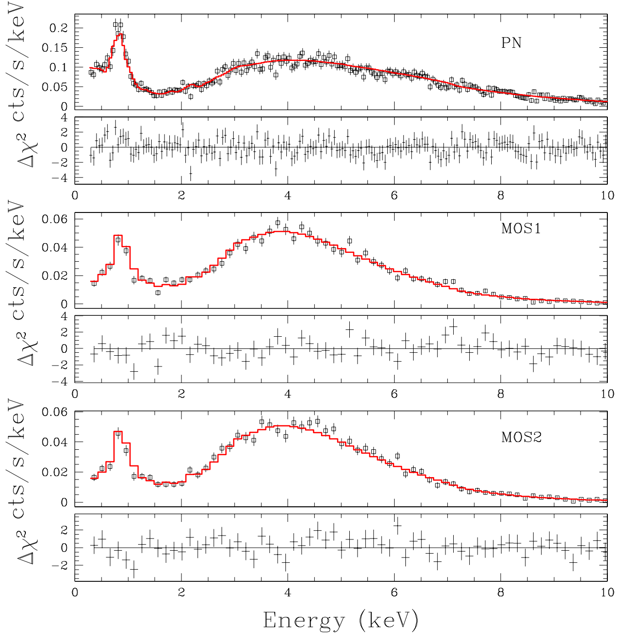
Fig. 2.— XMM- Newton EPIC spectra of the nucleus (15'' extraction radius) of NGC 4258 for the observation of 2000-12-08. Data were “grouped” by 10 pulse-invariant (PI) channels. PN, MOS1 and MOS2 data were fitted simultaneously with a model consisting of 2 power laws plus a thermal spectrum absorbed by intrinsic and Galactic gas ( N_H ) (see text). The best fit (solid line) and residuals (in units of sigmas) are shown for all instruments. These are the same data presented by Pietsch & Read (2002) (note that their Figures 2 and 5 report units of counts \text{cm}^{-2} \text{s}^{-1} \text{keV}^{-1} while they should read counts \text{s}^{-1} \text{keV}^{-1} , as in our plots, given that the spectra are convolved with the instrumental ancillary response function).
