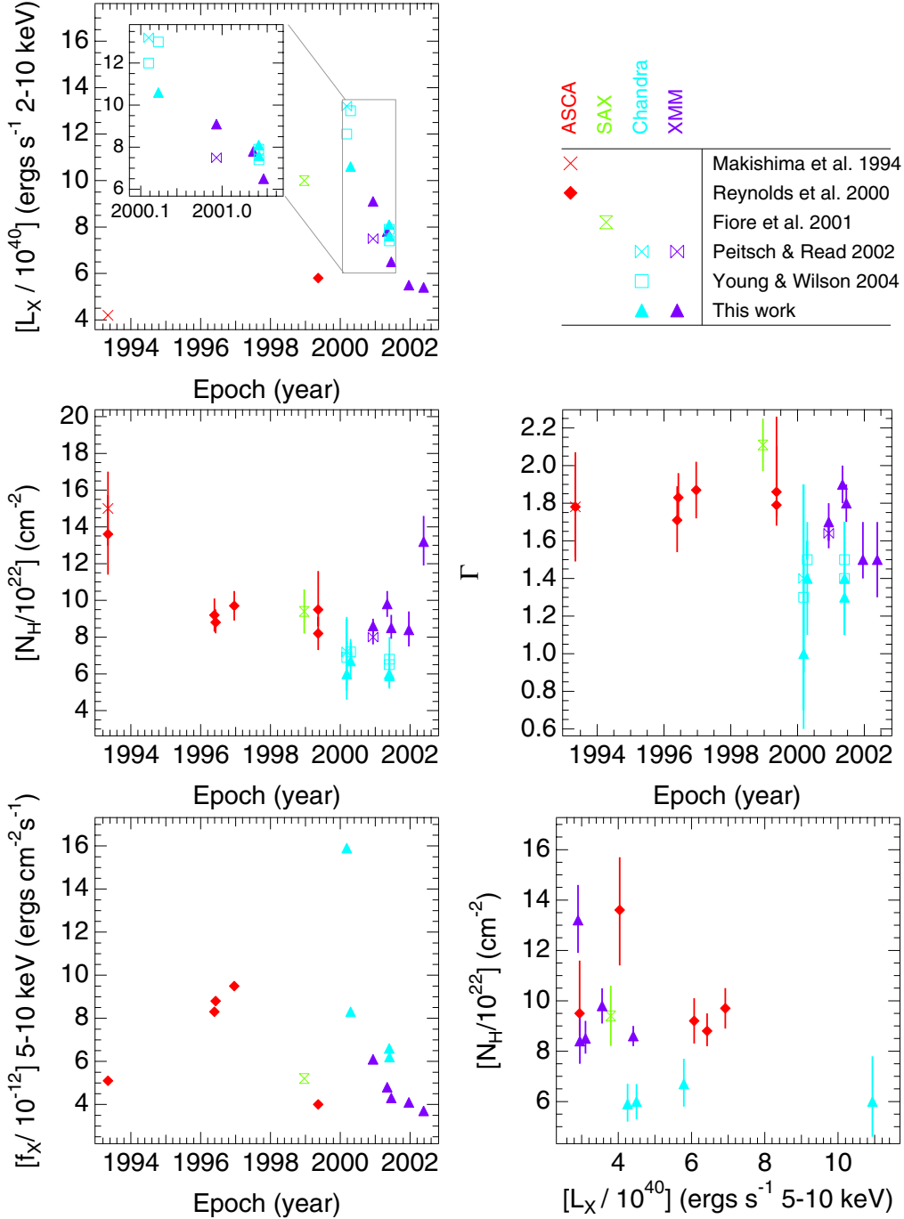
Fig. 14.— Time series of model column density ( N_H ), photon index ( \Gamma ), unabsorbed luminosity ( L_X ), and absorbed flux ( f_X ), as listed in Table 2. ( lower right )— Plot of N_H vs hard L_X , which tracks the hard f_X closely. No correlation is apparent, indicating that variations in flux are intrinsic to the central engine. Color is used to indicate mission while symbol type is used to code the reporting authors. Each dataset has been processed by more than one team. Plots of L_X (2-10 keV) and f_X (5-10 keV) are more sparse than plots of N_H and \Gamma because no single band is used throughout the literature.
