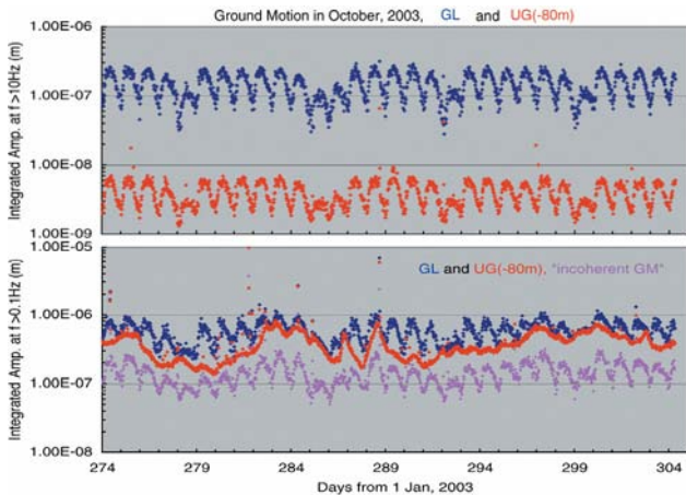
Figure 8: Integrated amplitude of ground motion measured at the KEK site on the surface (GL) and underground (UG) at 80 m depth.
