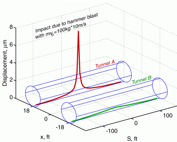
Figure 5: Impact due to a hammer blast with 100 kg*10m/s initial momentum in the 1 st tunnel and response in the 2 nd tunnel simulated with 3D code SASSI.
