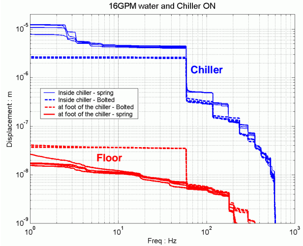
Figure 6: Vibration measured on an NLCTA water chiller and on the floor near the support with the chiller mounted rigidly, and with it placed on soft 3 Hz springs.
