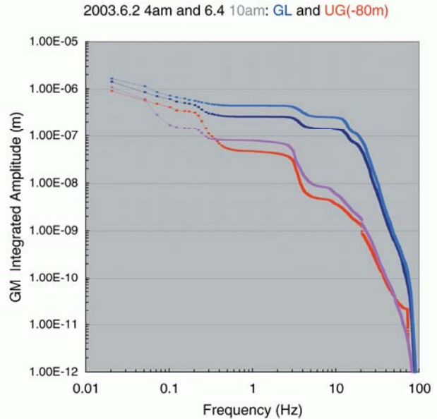
Figure 9: Integrated spectrum of ground motion measured at the KEK site on the surface and underground.
