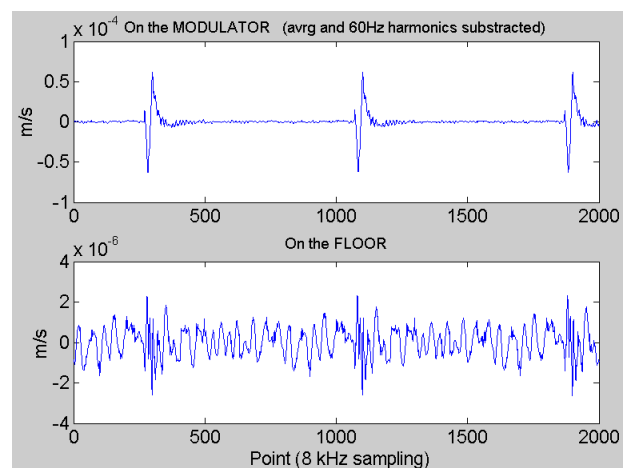
Figure 3: Vibration measured directly on the modulator (top plot), and on the floor near the modulator (bottom). The 60 Hz harmonics are removed for clarity.
