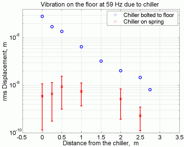
Figure 7: Vibration at 59Hz measured near the NLCTA water chiller when it is bolted to the floor and when placed on soft springs, averaged on several measurements.
