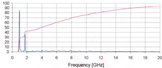
Figure 1. HOM calculation for a 952 MHz PEP-II style RF cavity with an increased bore.
