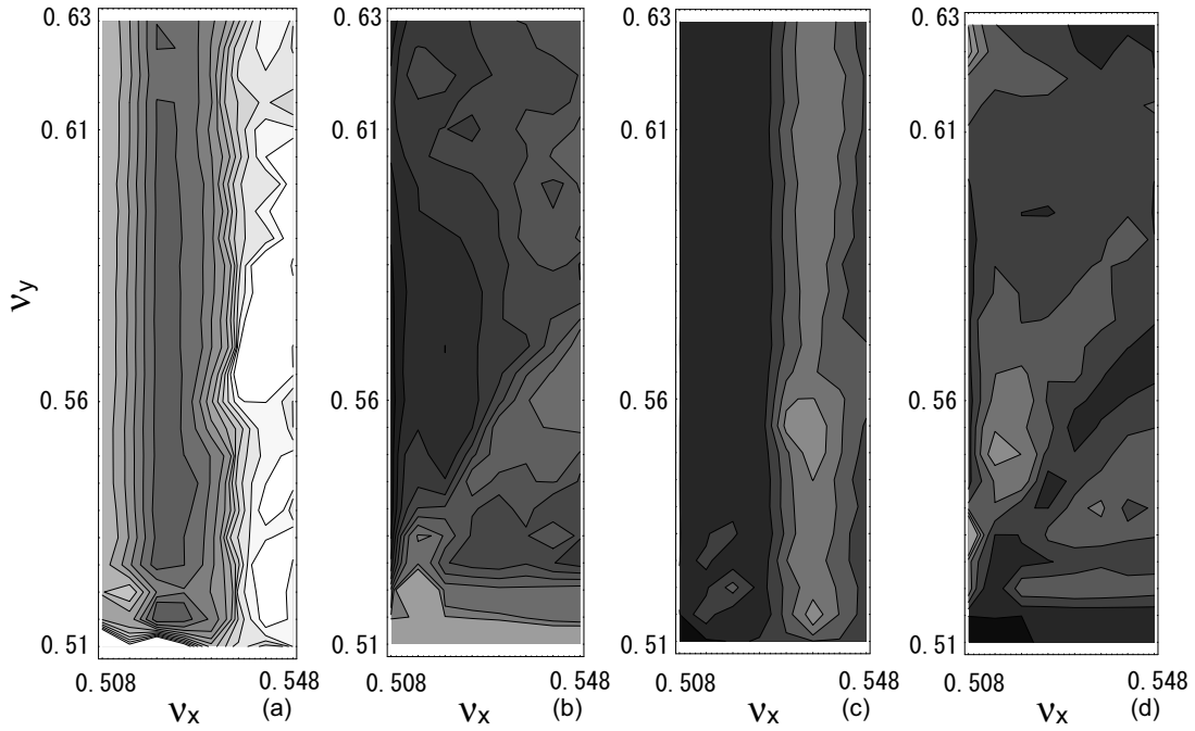
FIG. 7: Beam size and kurtosis in x - y tune space for crossing angle of 11 mrad. The horizontal and vertical beam sizes are depicted in Pictures (a) and (b), respectively. The horizontal and vertical kurtosis are depicted in Pictures (c) and (d), respectively. The contour lines are drawn every 10 \mu\text{m} , 1 \mu\text{m} and 1 for horizontal, vertical beam size and kurtosis, respectively, and lighter gray corresponds larger beam size and kurtosis.
