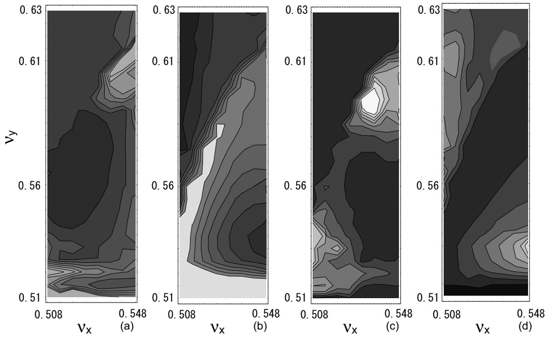
FIG. 6: Beam size and kurtosis in x - y tune space for zero crossing angle. The horizontal and vertical beam sizes are depicted in Pictures (a) and (b), respectively. The horizontal and vertical kurtosis are depicted in Pictures (c) and (d), respectively. The contour lines are drawn every 10 \mu\text{m} , 1 \mu\text{m} and 1 for horizontal, vertical beam size and kurtosis, respectively, and lighter gray corresponds larger beam size and kurtosis.
