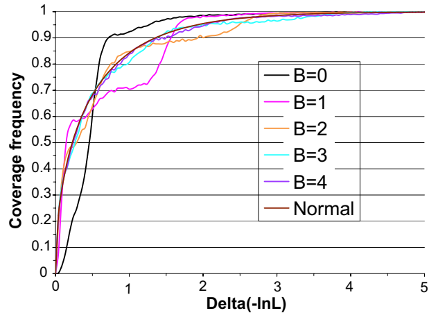
Figure 6: Coverage frequency as a function of \Delta for f = 1 , \sigma_f = 0.1 , b = 0.5 , \sigma_b = 0.1 . There are several curves corresponding to different numbers of expected signal events, B . The smoothest curve is the coverage in the high statistics (normal) limit.
