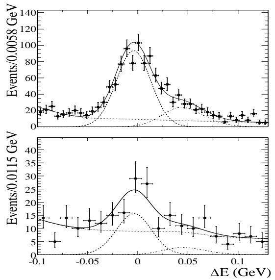
FIG. 1: Distributions of \Delta E for events enhanced in B \rightarrow D^0 K signal. Top: D^0 \rightarrow K^- \pi^+, K^- \pi^+ \pi^+ \pi^-, K^- \pi^+ \pi^0 ; bottom: D^0 \rightarrow K^- K^+, \pi^- \pi^+ . Solid curves represent projections of the maximum likelihood fit; dashed, dashed-dotted and dotted curves represent the B \rightarrow D^0 K , B \rightarrow D^0 \pi and background contributions.
