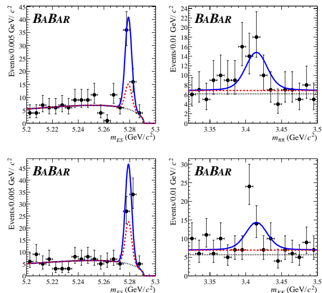
FIG. 1: Extraction of the signal yield for \chi_{c0} \rightarrow \pi^+\pi^- (top) and \chi_{c0} \rightarrow K^+K^- (bottom). Left: m_{ES} distribution; right: m_{\chi_{c0}} distribution. Dots with error bars represent the data; lines represent projection of the fitted functions for the three contributions: combinatorial background (dotted), peaking + combinatorial background (dashed), signal + backgrounds (solid).
