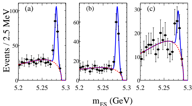
FIG. 1: Distributions of m_{ES} for B^- \rightarrow D^{*0}K^{*-} : (a) all modes; (b) D^{*0} \rightarrow D^0\pi^0 modes; (c) D^{*0} \rightarrow D^0\gamma modes.
