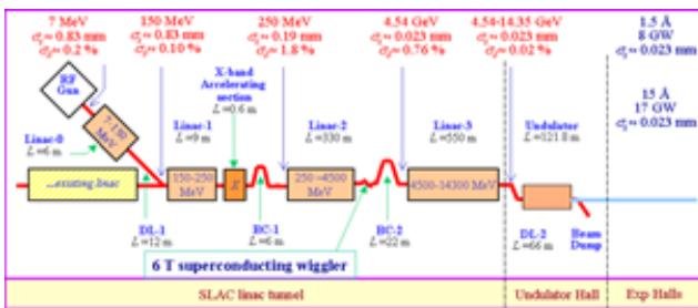
Figure 2. Schematic of LCLS accelerator systems, listing bunch length \sigma_z and energy spread \sigma_\delta at each stage of compression
