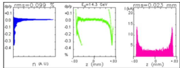
Figure 3. Longitudinal phase space of the electron bunch, compressed to 230 fsec
