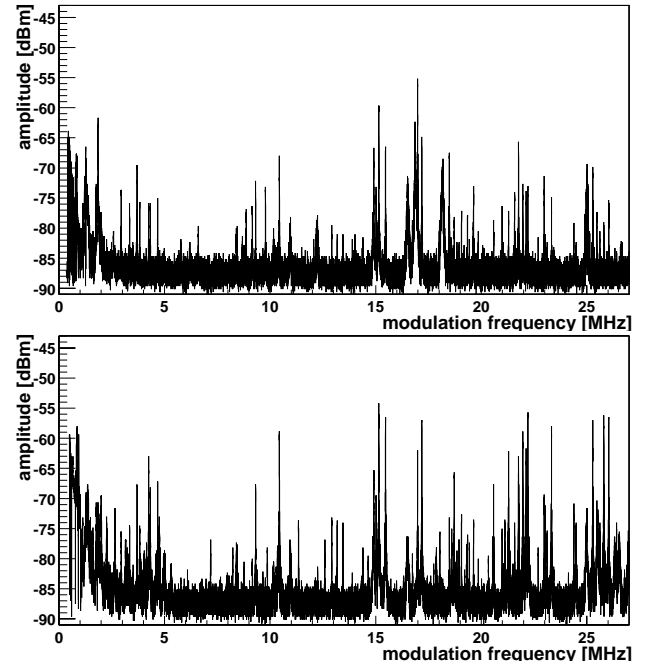
Figure 5: Beam oscillation amplitude after 200 \mu\text{s} charge modulation as function of the modulation frequency. Upper plot: horizontal scan. Lower plot: vertical scan.
