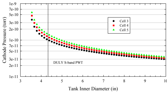
Figure 3: Pressure in the polarized PWT gun for increasing tank diameter and fully circumferential sieve.
