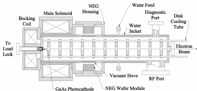
Figure 1: Schematic of the DULY S-band integrated PWT linac as modified for polarized electron production.
