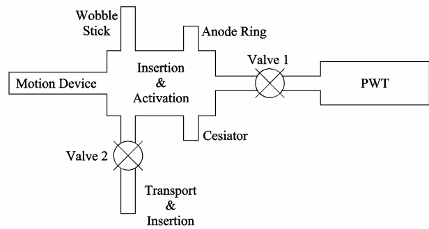
Figure 4: Block diagram of the load lock system.
