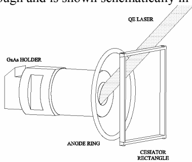
Figure 6: Schematic orientations of the anode ring, cesiator and QE diagnostic laser, showing that the laser clears the anode ring and the cesium dispensers.
