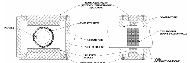
Figure 2: Schematic showing the circumferential sieve layout including the NEG modules and vacuum housing.
