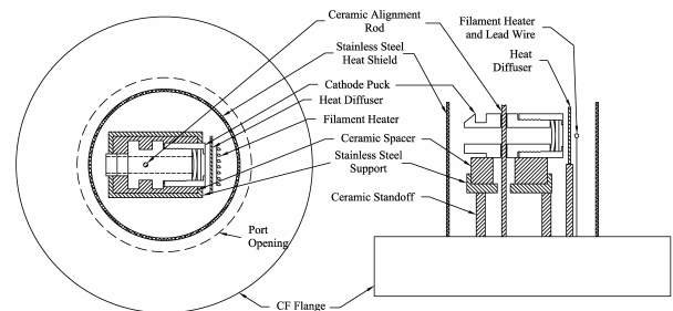
Figure 5: Schematic of the vacuum based heater used to activate the GaAs cathode.
