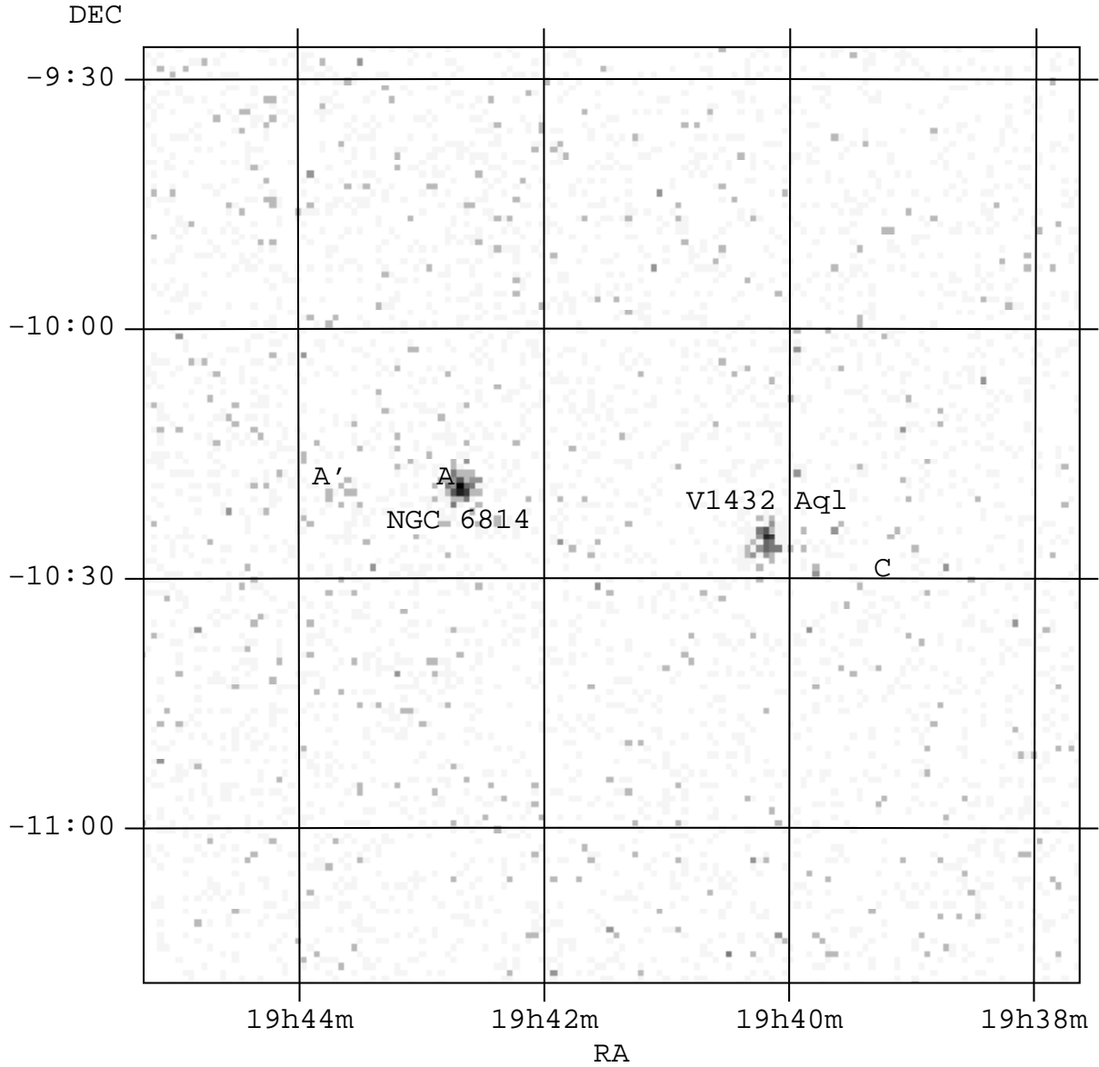
Fig. 1.— The ROSAT All-Sky Survey image of the region containing NGC 6814 (detected at 0.36 \text{ ctss}^{-1} ) and V1432 Aql ( 0.32 \text{ ctss}^{-1} ), marked with the pointing positions (A and C) used in our RXTE observing campaign. Also marked (A') is the intended pointing position (see text).
