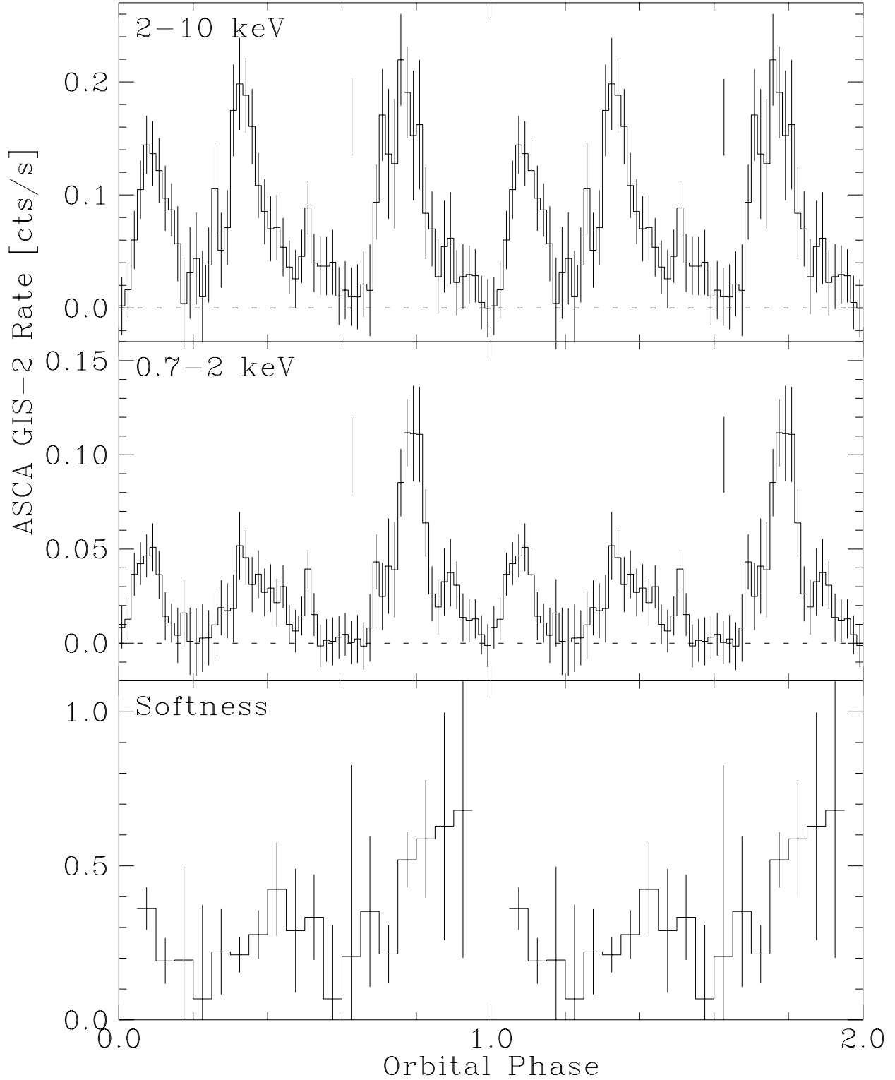
Fig. 9.— ASCA GIS-2 light curves in two energy bands folded on the orbital period using ephemeris (1) (120 bins per cycle, or \sim 100 s per bin) and the softness ratio ( [0.7\text{--}2 keV count rate]/ [2\text{--}10 keV count rate], 20 bins per cycle), plotted twice. The vertical lines in the upper two panels indicate the expected orbital phase of the optical spin minimum during this observation, according to ephemeris (2).
