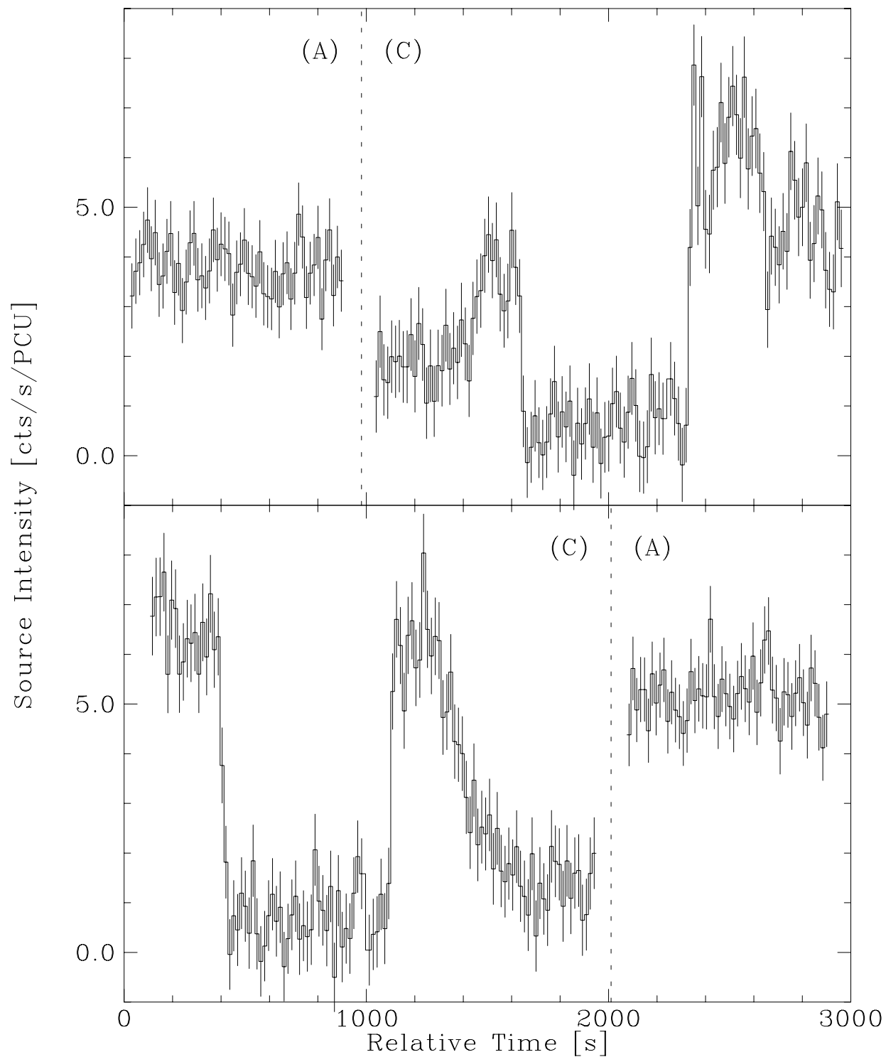
Fig. 2.— Light curves obtained at pointing positions A and C during the 1st and the 9th RXTE PCA observations, likely dominated by the NGC 6814 and V1432 Aql, respectively. The bin size is 16 s, and time 0 corresponds to 1998 May 18 at 12:58:00 UT (top) and 1998 June 19 at 19:21:40 UT (bottom), respectively.
