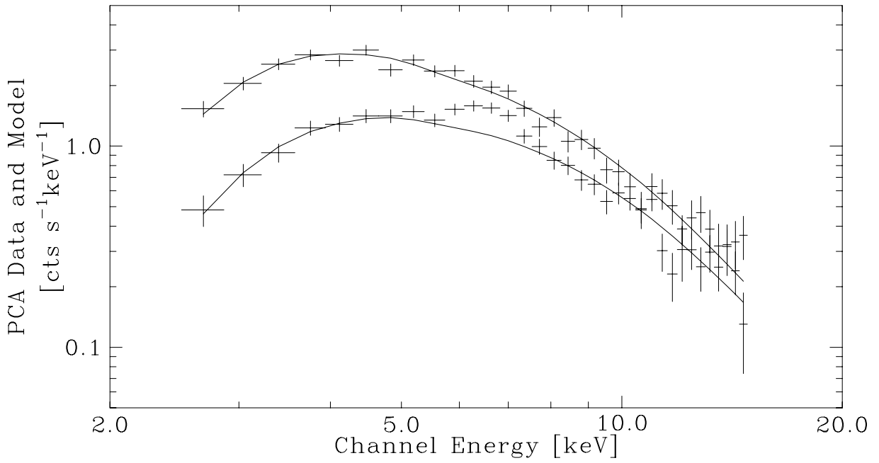
Fig. 3.— The spectra of NGC 6814 (brighter) and V1432 Aql (fainter) from the 1st RXTE PCA observation. Best-fit continuum models are also plotted, even though an Fe K \alpha is clearly required for the latter.
