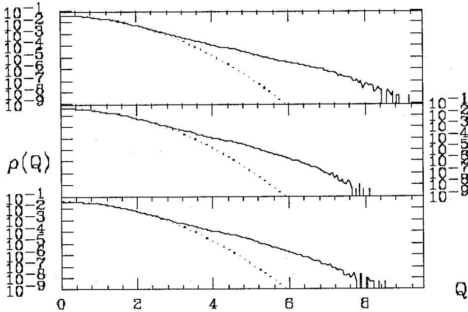
Figure 4: Transverse distribution for three values of R_2 : R_2 = 0 (bottom), R_2 = 0.01 (middle) and R_2 = 0.1 (top). The horizontal axis is Q , the normalized distance from the origin, and the vertical the distribution in Q . The data was taken for 100 particles and through 2 \times 10^6 turns. Parameters: \nu_x = 0.15 , \nu_s = 0.085 , T_e = 200 and T_x = 400 , \eta = 0.1 , R_1 = 0.5 and L = 3 .
