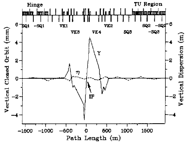
Figure 5. Vertical crossing angle at the IP.
