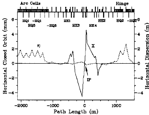
Figure 4. Horizontal crossing angle at the IP.
