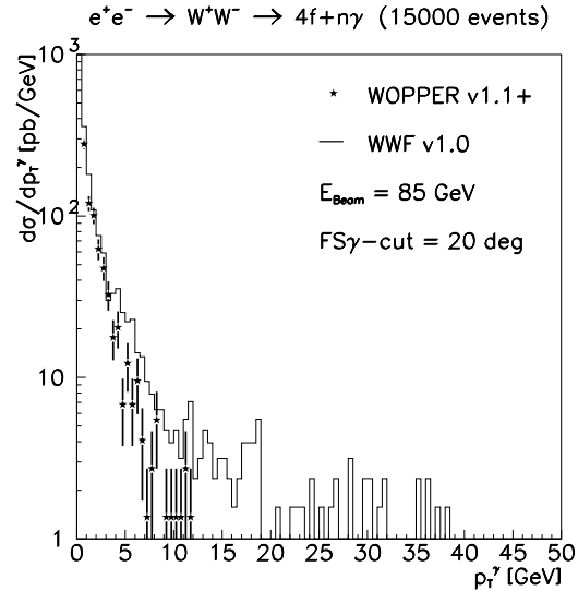
Figure 3. Same as figure 2, but for the photonic transversal momentum p_T^\gamma .
