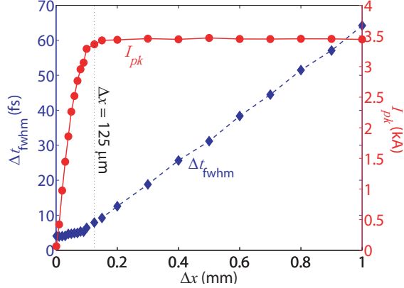
FIG. 3: Peak current (red ●) and fwhm pulse length (blue ◇) of unspoiled electrons vs. slot half-width, \Delta x . The minimum e^- pulse at full current is 8 fs ( \Delta x = 125 \mu\text{m} ).
