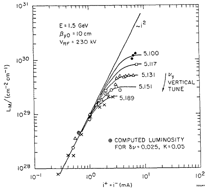
FIG. 6--Luminosity vs beam current for various values of the vertical time.
