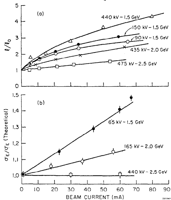
FIG. 3--Fraction increase vs beam current of (a) bunch length and (b) energy spread derived from the quantum lifetime formula. The numbers of the curves give the RF voltage and beam energy.
