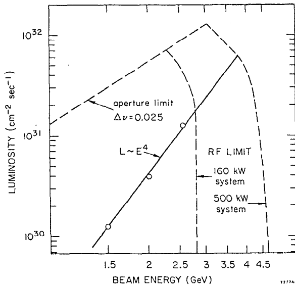
FIG. 5--Luminosity vs energy. The dashed lines show the design limits for both the present RF system, and for the new 500 kW system now under construction. The open circles are measured values.
