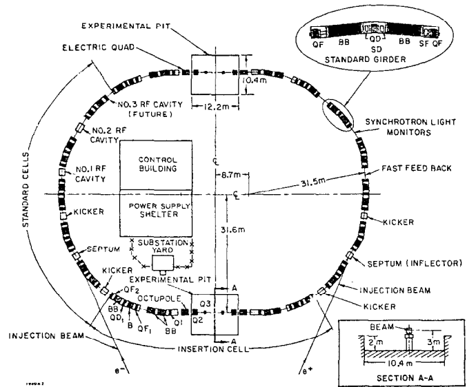
FIG. 1--Layout of SPEAR.
