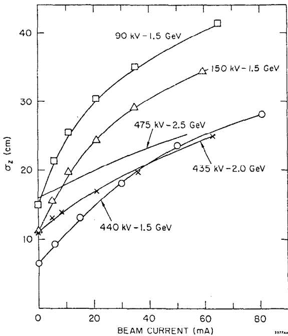
FIG. 2--Bunch length (standard deviation) vs beam current for various values of RF-accelerating voltage and circulating-beam energy.
