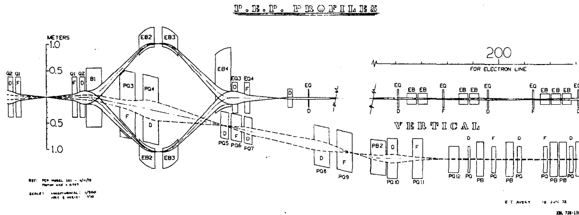
Fig. 1. Profiles for a PEP machine design example. The scale is longitudinally 1/200, and horizontally and vertically 1/10. Bending magnets are marked with B, quadrupoles with Q or with F (focussing in that plane) and D (defocussing in that plane). The electron line is often indicated by E, the proton line by P.
