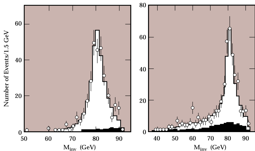
Reconstructed W mass peaks. On the left, one W decays to a charged lepton and a neutrino while the other decays into a pair of quarks. On the right, both W's decay into quark pairs. These data come from the L3 Collaboration; the solid lines are fits to the data and the black areas represent background events.
