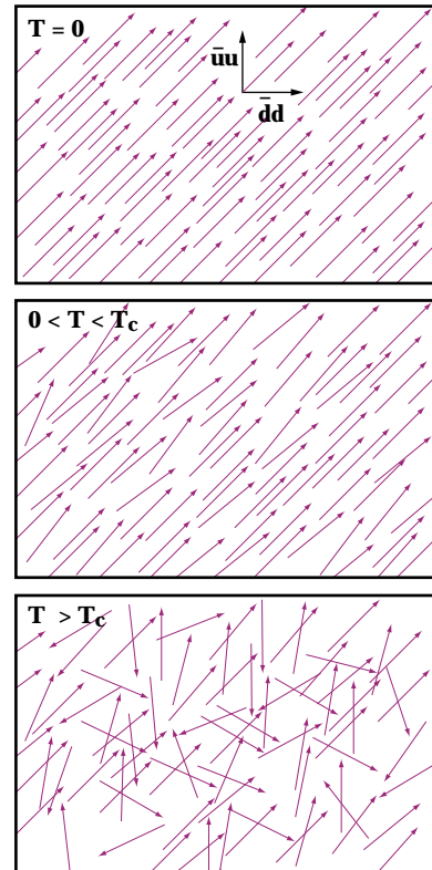
Melting the Vacuum. (Top) The QCD vacuum is a condensate. At each location are quark-antiquark pairs whose type must be specified by an arrow indicating what fraction of the pairs are u\bar{u} versus d\bar{d} versus u\bar{d} versus d\bar{u} . Only two of these four directions are shown. The central property of a condensate is that all the arrows are aligned. (Middle) At non-zero temperatures, the arrows describing the condensate begin to undulate. These waves can equally well be described as a gas of particles, called pions. (Bottom) As the temperature increases, the waves on the condensate become more and more violent. Above some critical temperature, the arrows are completely scrambled, and the condensate has melted.
