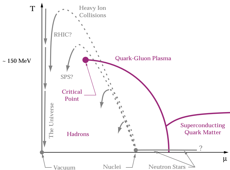
Phases of QCD as a function of temperature and \mu , a quantity that is a convenient measure of the net quark density, namely the density of quarks minus that of antiquarks. The vacuum is at the bottom left; nuclei have non-zero net quark density. Squeezing nuclei without heating them pushes matter to the right on the diagram, while heating matter pushes it up. The colored line separating the quark-gluon plasma from the hadronic phase ends at a critical point.
