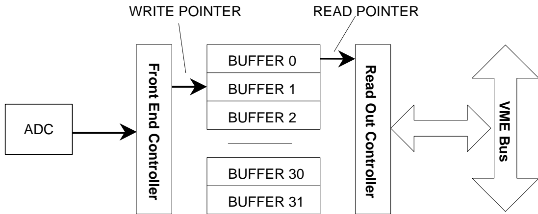
Fig. 2.7: Multi-Event Buffer: Write pointer and Read pointer
