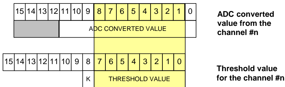
Fig. 2.6: Zero suppression (Bit 8 of Bit Set 2 Register =1)
