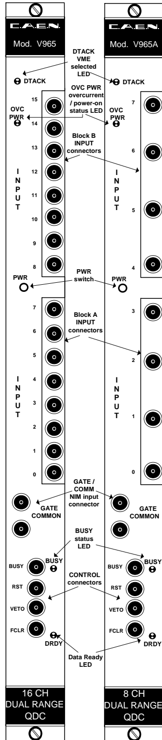
Fig. 3.1: Model V965/V965A front panels
