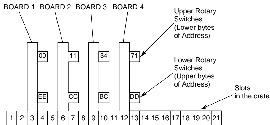
Fig. 4.4: MCST/CBLT Addressing Example
