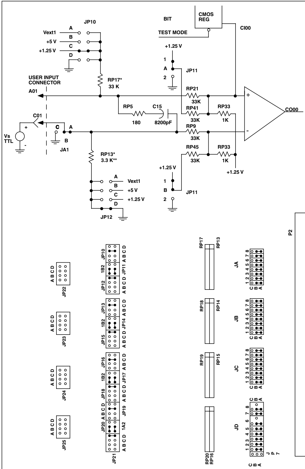
Figure 5.5-8. Jumper Configuration and Typical Input Circuit for Voltage Sourcing, TTL Neg True
