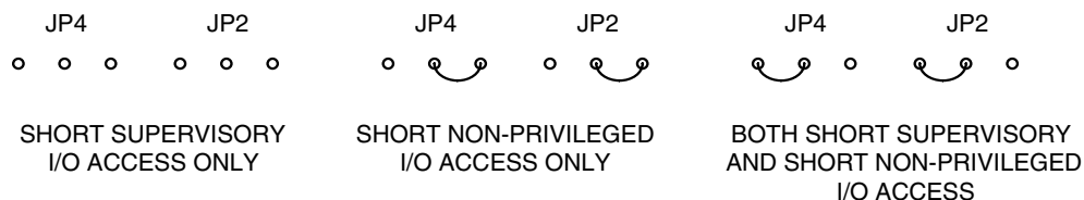
Figure 5.4-1. Address Modifier Selections
