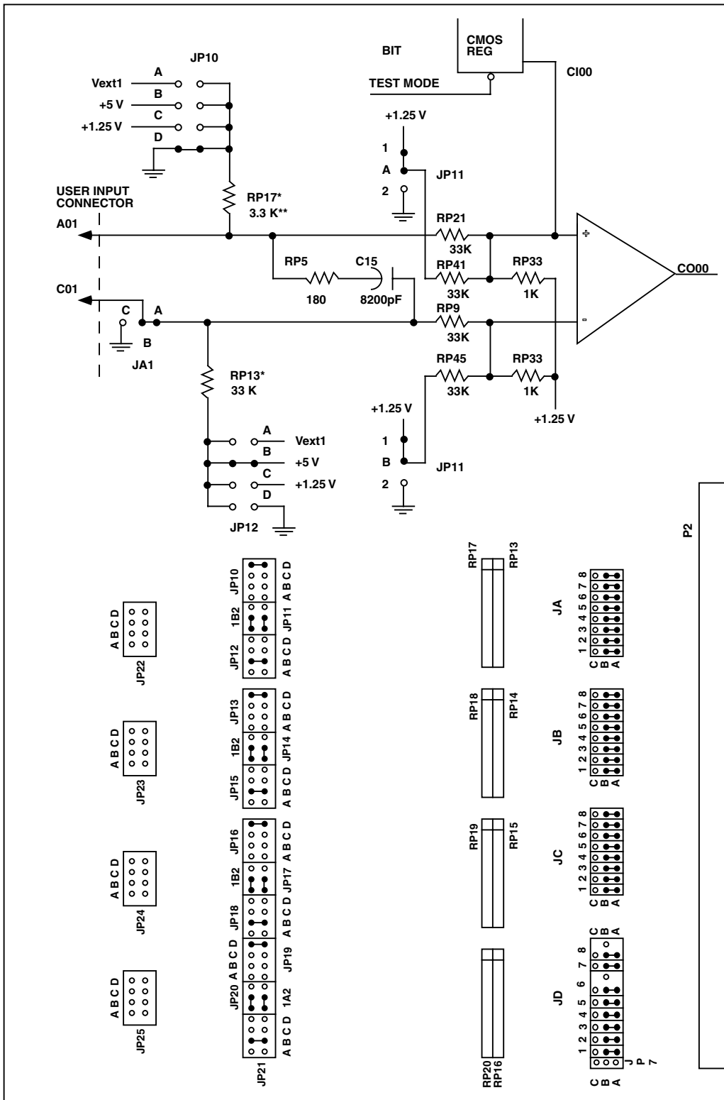
Figure 5.5-1. Jumper Configuration and Typical Input Circuit for Differential Inputs
