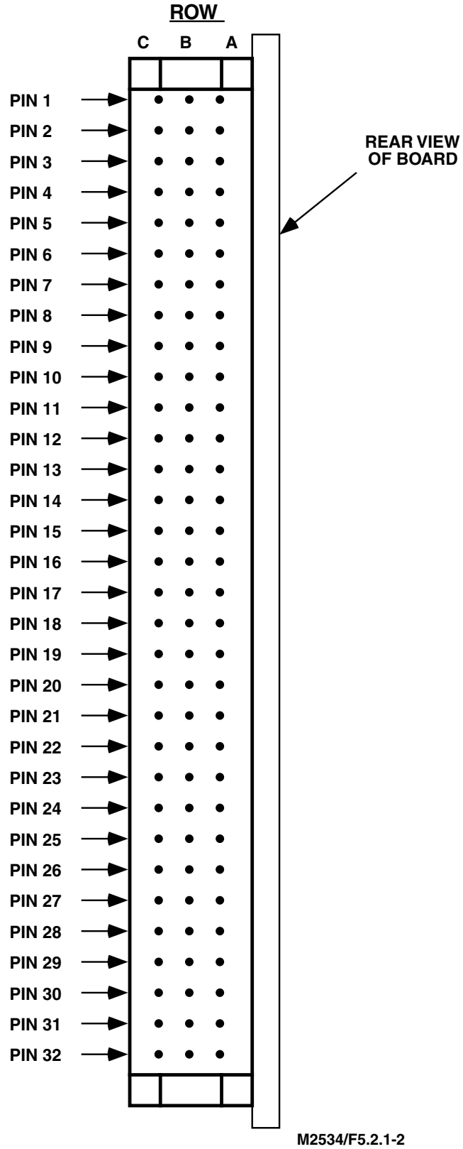
Figure 5.2.1-2. P2 Connector Pin Layout
