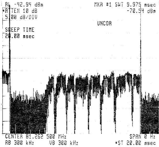
Figure 5: Time dependence of the amplitude of the vertical sideband at 10f_0 - v_y , over a period of 20 ms starting at injection (left hand peak).
