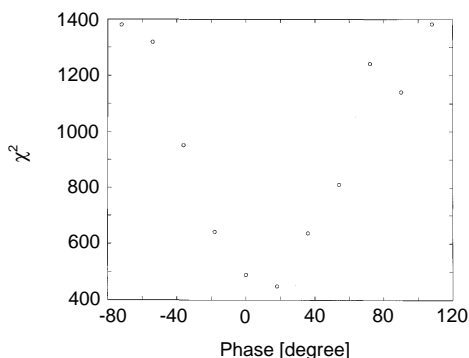
Figure 6: The phase \phi_0 between the electron bunch and the long-range wakefield is indicated by a minimum \chi^2 of the fitted solution.
