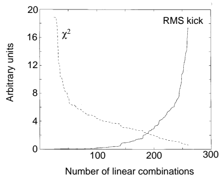
Figure 4: The \chi^2 and the RMS kick found by SVD as a function of the number of linear combinations that are included into the solution. The \chi^2 can be greatly reduced with just a few kick combinations. If too many combinations are included, unphysically strong kicks are introduced that reduce the \chi^2 only slightly.
