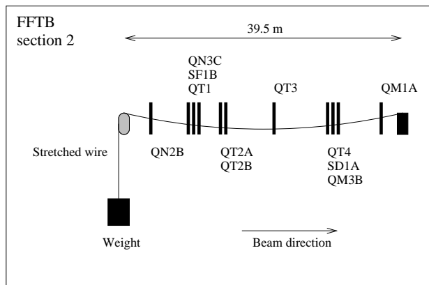
Figure 1: Illustration of the wire in section 2. The wire is stretched with a weight of about 35 kg at its upstream end. The beamline elements are distributed along the wire, sometimes grouped in doublets or triplets. Each element has three wire position monitors attached to it.
