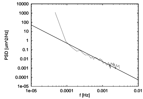
Figure 5: Spectrum of uncorrelated vertical magnet motion obtained in section 2 of the Final Focus Test Beam at SLAC. The straight line corresponds to an ATL spectrum with a proportionality constant A = 2 \cdot 10^{-8} \mu\text{m}/(\text{m} \cdot \text{s}) and distance L = 10 m.
