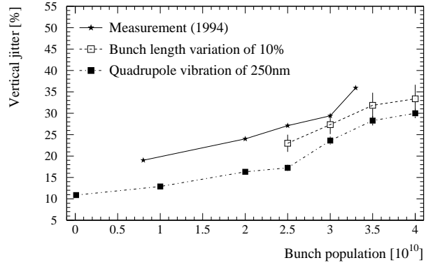
Figure 2: Vertical beam jitter in percentage of the beam size as a function of the bunch population. The solid curve shows the measured rms positron-orbit variation at high-beta points in the SLC final focus, averaged over data from 1994. The dashed-dotted curve presents simulation results for an uncorrelated rms quadrupole vibration of 250 nm. Finally the dashed curve shows simulation results for an emittance-optimized linac with an rms bunch length variation of 10%. All simulation results refer to the end of the linac.
