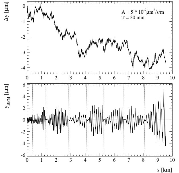
Figure 1: Example of ATL-like alignment drifts. The upper plot shows the displacements of quadrupoles, RF-structures and BPM's after 30 minutes with an A-coefficient of 5 \times 10^{-7} \mu\text{m}^2/\text{sec}/\text{m} . The alignment was flat initially. The lower plot shows the corresponding trajectory offsets y_{BPM} at the BPM's. The dotted lines indicate the locations of trajectory feedbacks where y and y' are corrected back to zero. Thus the size of coherent betatron oscillations is constrained.
