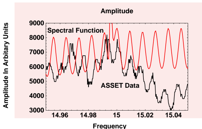
Fig. 5: Fine details of the observed spectrum, compared to theoretical predictions. The mode spacing is slightly smaller than predicted which is compatible with the observation of a somewhat delayed occurrence of the recoherence peak in the ASSET-wakefield measurements [1].
