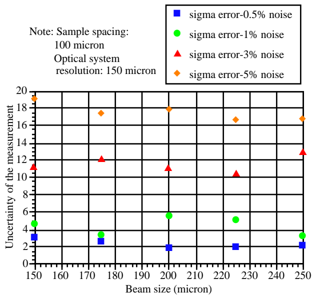
Figure 2. The uncertainty of beam size measurement with noise and optical smear.
