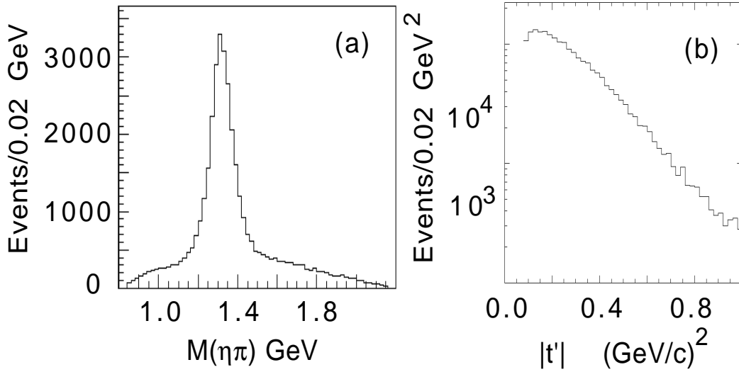
Figure 1: (a) The \eta\pi^- effective mass distribution. (b) Distribution of |t'| = |t| - |t|_{\min} .
