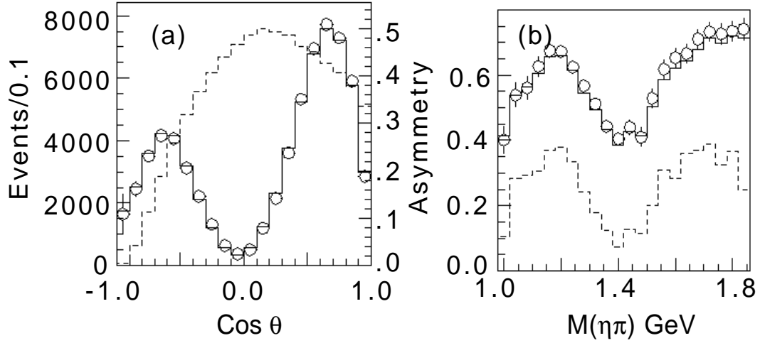
Figure 2: The open circles show (a) the acceptance-corrected distribution of the cosine of the decay angle in the Gottfried-Jackson frame for events with 1.22 < M(\eta\pi^-) < 1.42 \text{ GeV}/c^2 , and (b) the uncorrected forward-backward decay asymmetry as a function of M(\eta\pi^-) . The asymmetry = (F - B)/(F + B) , where F(B) is the number of events for which the \eta 's momentum is forward (backward) in the Gottfried-Jackson frame. The solid histograms in (a) and (b) show the values predicted by the PWA fit to the data. The dashed curve and the right-hand scale in (a) show the average acceptance in this mass region. The dashed curve in (b) shows the acceptance-corrected asymmetry.
