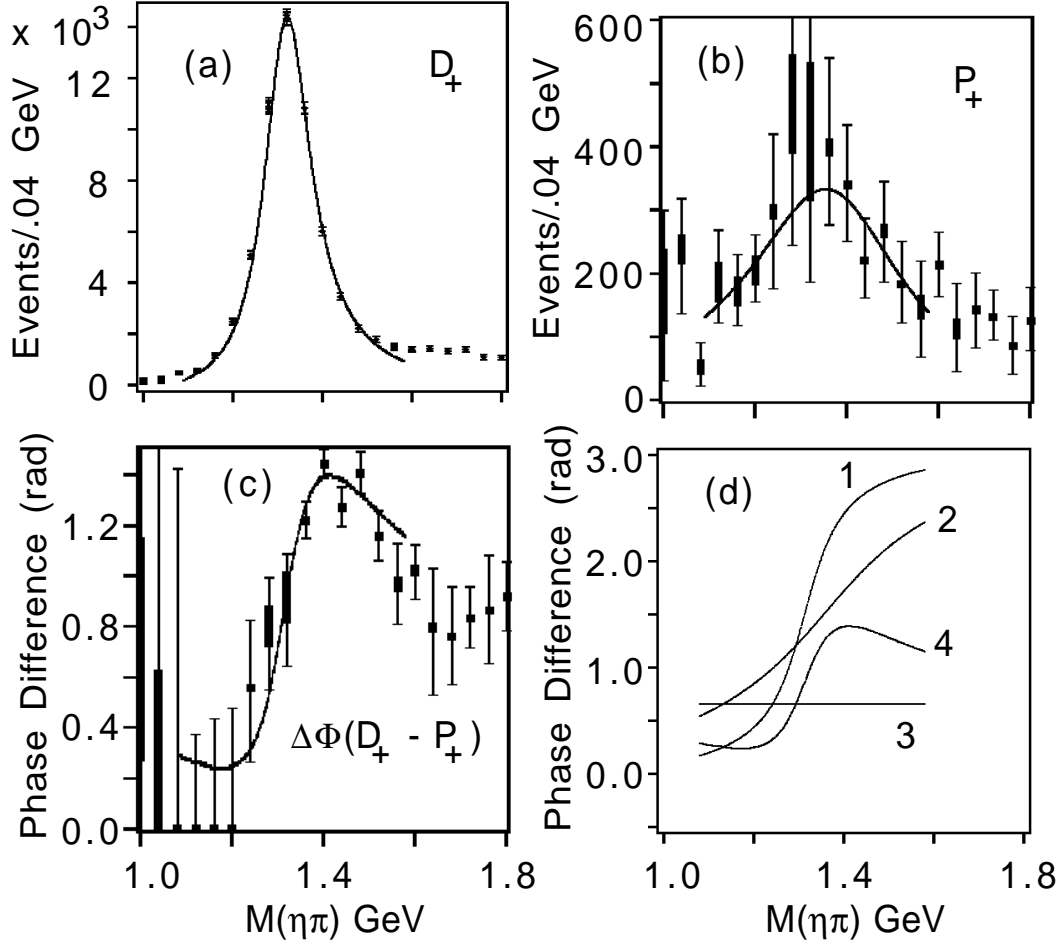
Figure 3: Results of the partial-wave amplitude analysis. Shown are (a) the fitted intensity distributions for the D_+ , (b) the P_+ partial waves, and (c) \Delta\Phi(D_+ - P_+) , their phase difference. The range of values for the eight ambiguous solutions is shown by the central bar and the extent of the maximum error is shown by the error bars. Also shown as curves in (a), (b), and (c) are the results of the mass dependent analysis described in the text. The lines in (d) correspond to (1) the fitted D_+ Breit-Wigner phase, (2) the fitted P_+ Breit-Wigner phase, (3) the fitted D_+ - P_+ relative production phase, and (4) the overall D_+ - P_+ phase difference as shown in (c), but with a different scale.
