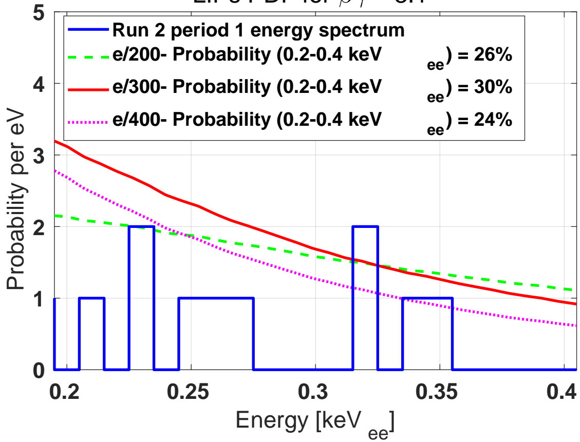
LIPs PDF for \beta\gamma = 3.1
