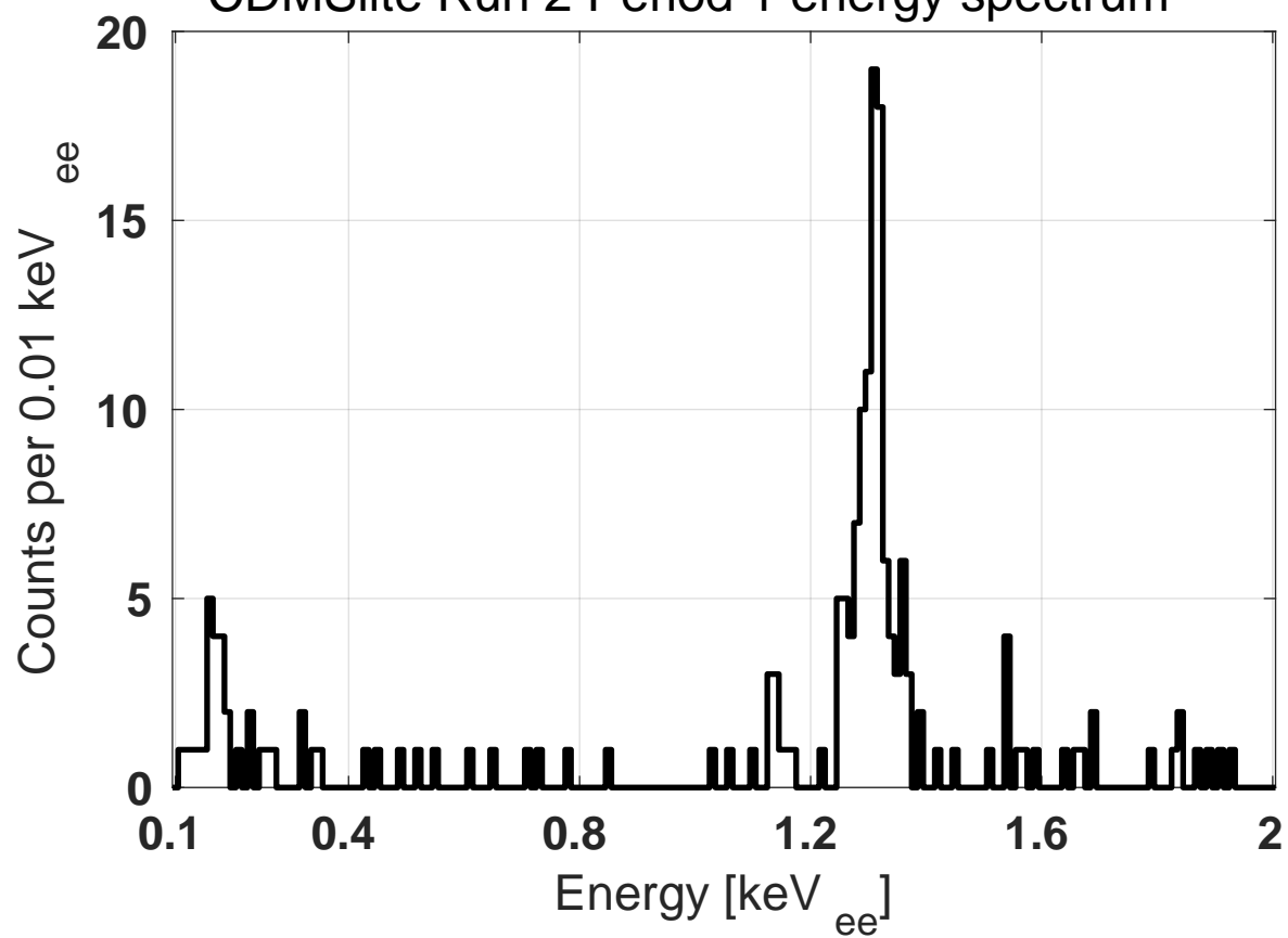
CDMSlite Run 2 Period 1 energy spectrum
