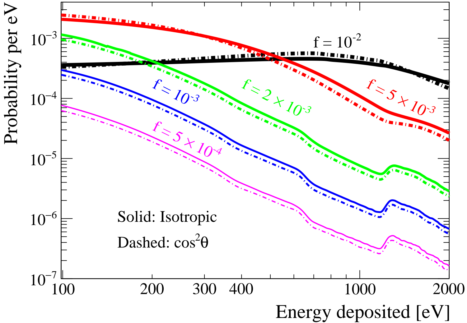
LIPs PDF (mass = 100 MeV, \beta\gamma = 3.1 )
