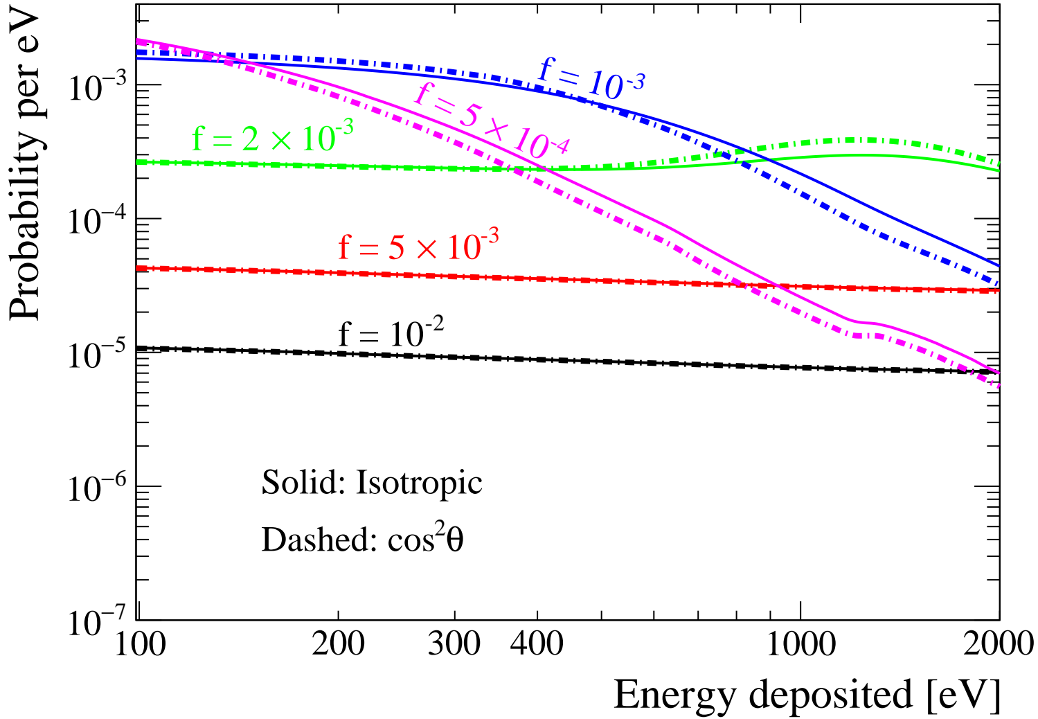
LIPs PDF (mass = 100 MeV, \beta\gamma = 0.1 )
