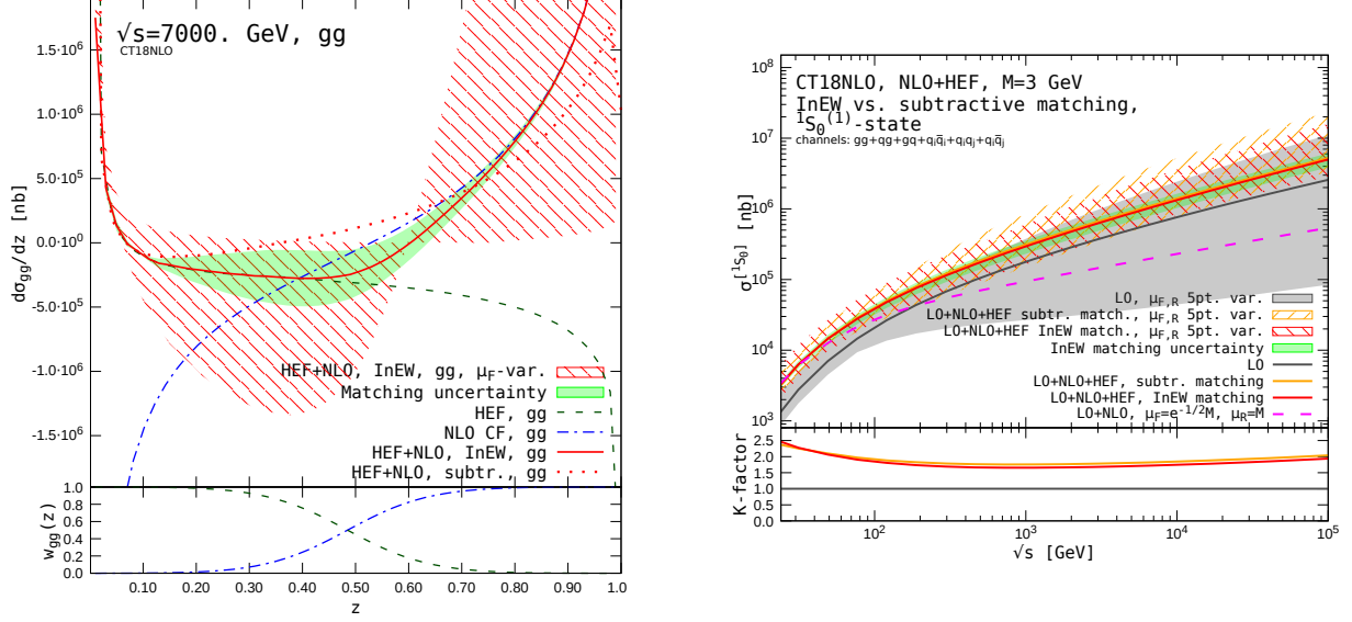
FIG. 7: Left panel: the integrand of the total \eta_c hadro-production cross section as function of z = M^2/\hat{s} in the gg -channel. Dashed line – DL HEF contribution, dash-dotted line – NLO CF contribution, solid line – their matching, according to the Eq. (10), the weight function is shown in the inset. Right panel: The total cross section of hadro-production production of the c\bar{c} [^1S_0^{(1)}] -state as function of \sqrt{s_{pp}} . Plots adopted from the Ref. [186].
