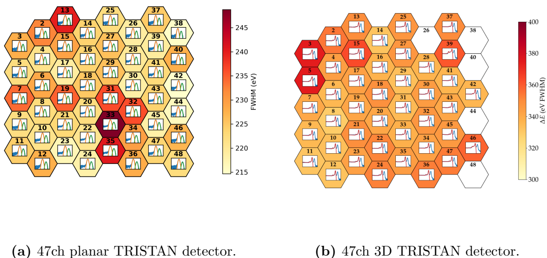
Figure 34: Pixel maps of the 47-pixel TRISTAN detector (planar and 3D design) in the KATRIN monitor spectrometer. The color bar indicates the energy resolution of the individual pixels. The plot insets show typical energy spectra ( ^{55}\text{Fe} calibration spectra for the planar detector and ^{83\text{m}}\text{Kr} spectra for the 3D detector). The spectra were fit with suitable functions. For the 3D design, five pixels did not work properly and were excluded from the analysis; they are marked here in white.
