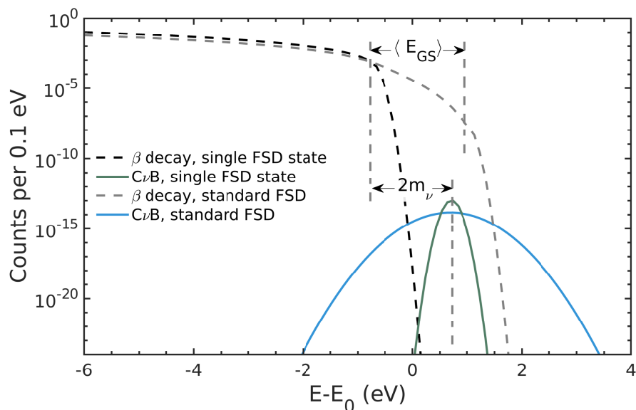
Figure 13: Simulation of the effects of the molecular final-state distribution (FSD) on the differential spectra from \beta decay and from relic-neutrino capture, assuming m_\nu = 0.7 eV and \eta = 1 ; details are in Ref. [111], from which this figure is adapted. Doppler broadening is included for all spectra. \langle E_{GS} \rangle \approx 1.7 eV is the mean energy of the electronic ground state.
