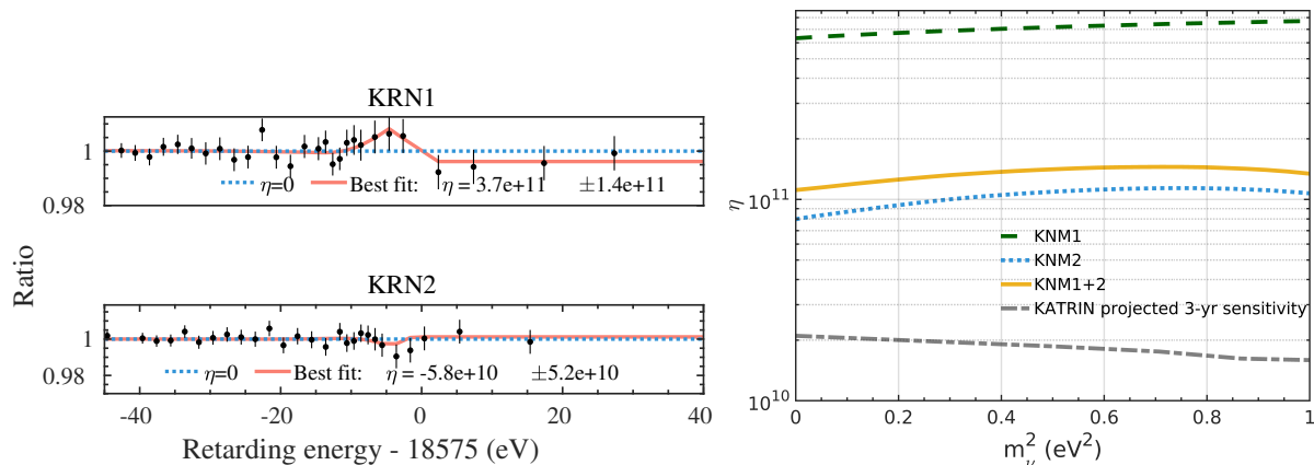
Figure 14: Left: Spectral ratio of the best fits for relic neutrinos with respect to the null hypothesis \eta = 0 for the first two measurement campaigns. The non-zero values of the best fit of \eta are both consistent with background fluctuations. Right: Exclusion contours for the relic-neutrino overdensity \eta at 99% C.L. for both measurement campaigns and their combination, and the projected final KATRIN sensitivity. Adapted from Ref. [111].
