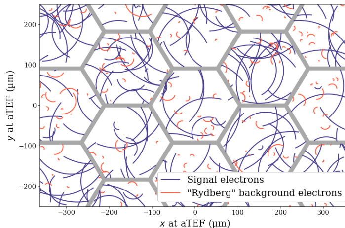
Figure 19: Simulation of signal (purple) and background (orange) electron tracks in a 2.4 T axial magnetic field with the angular distributions shown in Fig. 17 for a honeycomb-like aTEF structure with a side length of 100 \mu\text{m} , a wall thickness of 10 \mu\text{m} , and a depth of 400 \mu\text{m} . The tracking of an electron is stopped when it either hits the aTEF surface or when it reaches the full depth without any hit. Adapted with permission from Ref. [131].
