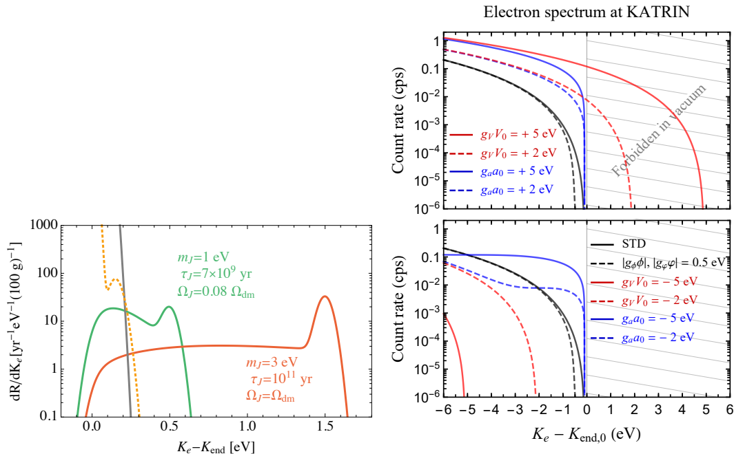
Figure 15: Left: Event rates for capture on tritium for neutrinos from Majoron decay J \rightarrow \nu\nu for m_J = 1 eV, \tau_J = 7 \times 10^9 yr, \Omega_J/\Omega_{\text{dm}} = 0.08 (green, solid) and m_J = 3 eV, \tau_J = 10^{11} yr, \Omega_J/\Omega_{\text{dm}} = 1 (red, solid) and natural \beta decay (gray, solid) with an electron energy resolution of 0.1 eV. For comparison, we plot the total rate for signal plus background for a Majorana relic-neutrino signal with m_\nu = 0.15 eV (yellow, dashed). Taken from [115]. Right: The integrated \beta -decay spectra at KATRIN in various types of media: scalar, pseudoscalar and two different vector and axial-vector potentials, with neutrino mass fixed to 0.1 eV. Taken from [117].
