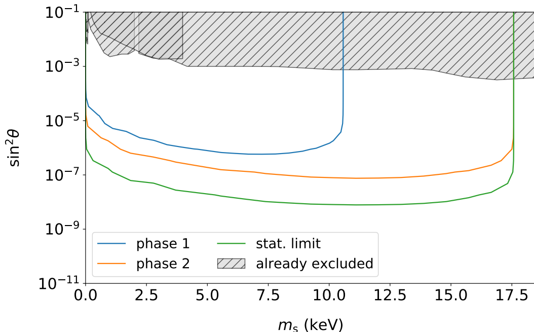
Figure 10: KATRIN sensitivity to keV-scale sterile neutrinos in different scenarios. The statistical limit assumes 10^{18} electrons over the full energy range, corresponding to a measurement time of one year at the full KATRIN source strength. Phase 1 denotes the first stage of TRISTAN operation with a reduced amount of TRISTAN modules (approx. 1000 pixels) and a lowered KATRIN source strength (0.3% of the nominal column density). The spectrum is scanned on an energy interval of 8 keV to 18 keV with a total measurement time of t_{\text{meas}} = 0.5 yrs. In the follow up stage (phase 2), the TRISTAN detector is operated with all 3500 pixels. The tritium spectrum is scanned on the full energy range at a reduced source activity of 2% of the nominal column density for t_{\text{meas}} = 1.0 yrs. The already excluded parameter space is based on Refs. [74, 89, 90, 91].
