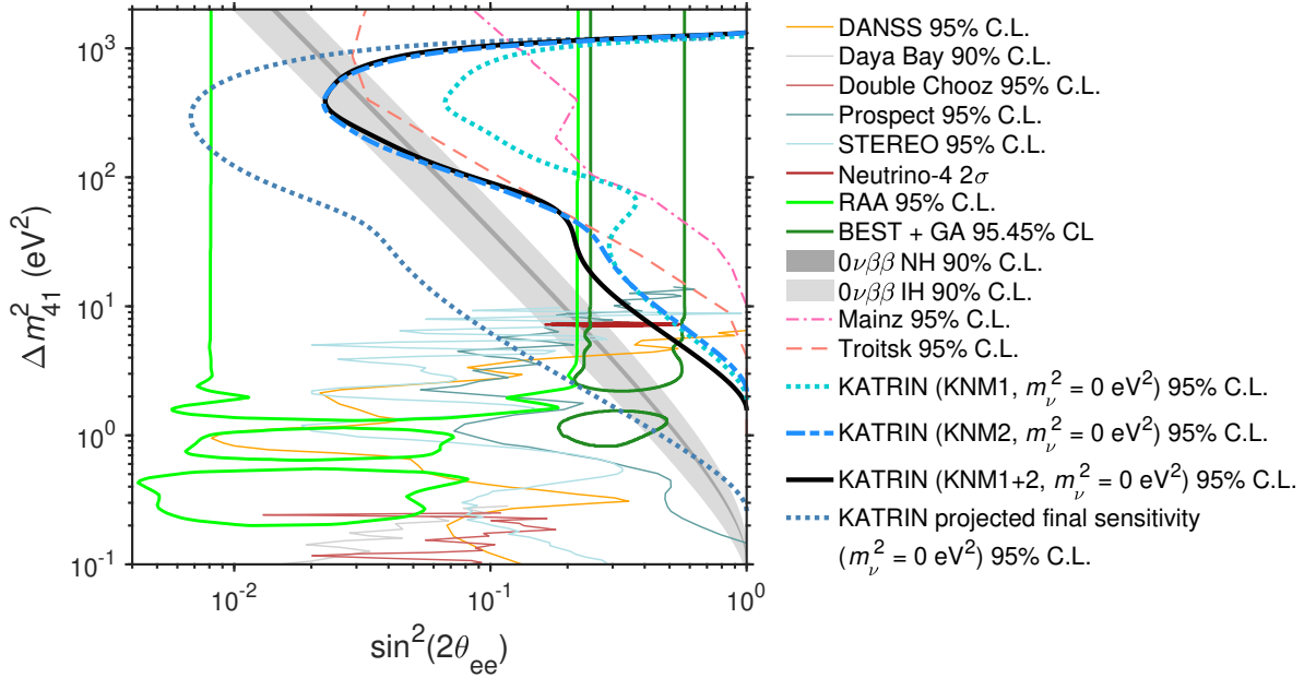
Figure 8: 95 % C.L. exclusion contours of the first and second KATRIN science run with m_\nu^2 = 0 \text{ eV}^2 , as well as the combined exclusion from both campaigns. The final sensitivity is given by the projection described in Ref. [72]. The second measurement is able to exclude a wider range than both the Mainz [74] and Troitsk [75] experiments for m_4^2 \lesssim 300 \text{ eV}^2 . Large \Delta m_{41}^2 can be excluded to a great extent for the solutions of the reactor antineutrino anomaly (RAA) and BEST+gallium (GA) anomalies [63, 66]. The combined analysis is in tension with the positive results claimed by Neutrino-4 [76] for \sin^2(2\theta_{ee}) \gtrsim 0.4 . KATRIN data improve the exclusion bounds set by short-baseline oscillation experiments for \Delta m_{41}^2 \gtrsim 10 \text{ eV}^2 [67, 68, 69, 70, 71]. Constraints from 0\nu\beta\beta with m_{\beta\beta} < 0.16 \text{ eV} are shown as gray bands [77, 78, 79]. Adapted from Ref. [73].
