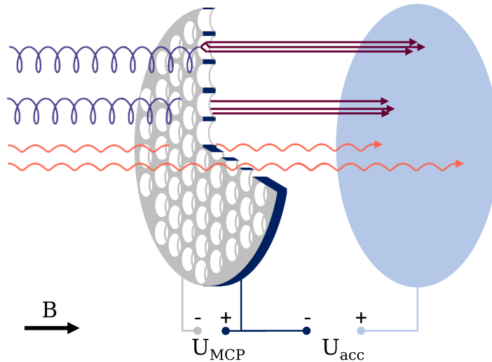
Figure 18: Principle of an MCP-based active transverse energy filter in front of the KATRIN detector (light blue) in a horizontal magnetic field B . Electrons with a small cyclotron radius (orange) pass the MCP without interaction and hit the detector. Electrons with a large cyclotron radius (purple) hit the MCP walls, giving rise to a cascade of secondary electrons (dark red) that is accelerated via U_{acc} towards the detector. Since the secondary electrons are produced with practically no transverse momentum, they follow the magnetic-field lines without a sizable cyclotron radius. Adapted with permission from Ref. [131].
