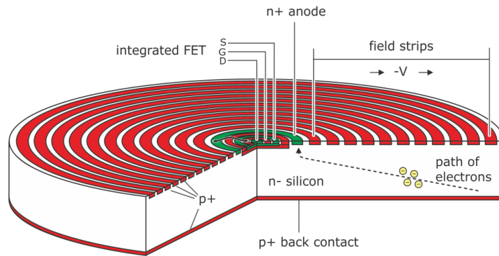
Figure 25: Schematic of a single pixel of the TRISTAN silicon drift detector, reproduced with permission from Ref. [139]. Electrons are guided by an electric field to the collecting n+ anode in the center of the detector, which is surrounded by several drift rings. The entrance window for radiation is on the opposite side (p+ back contact). The detector features an integrated field-effect transistor (FET) close to the anode which forms the first stage of the readout electronics.
