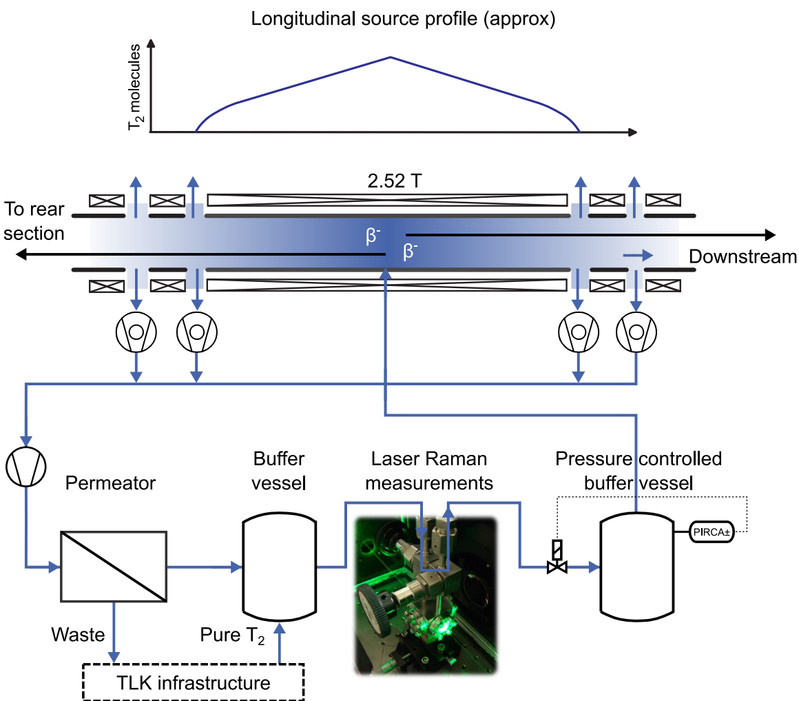
Figure 2: Simplified schematic of the windowless gaseous tritium source (WGTS) and tritium circulation loop. The temperature of the WGTS beam tube was 30 K in the first two campaigns [15, 1] and has been changed to 80 K for subsequent campaigns.
