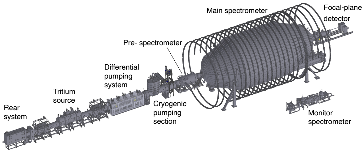
Figure 1: Engineering drawing of the KATRIN beamline.
