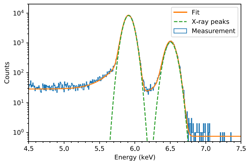
Figure 27: Energy spectrum of ^{55}\text{Fe} recorded with a 2 mm pixel-diameter SDD array at a temperature of -30^\circ\text{C} . The \text{MnK}\alpha line at 5.9 keV has an energy resolution of 139 eV FWHM and is clearly separated from the \text{MnK}\beta line at 6.5 keV. Two phenomenological functions similar to a hypermet [148] were used to fit the spectrum. Reproduced from Ref. [145].
