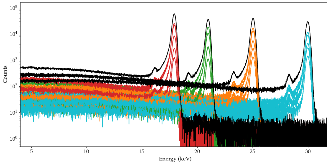
Figure 35: Energy spectra (wall electrons) measured with a 47-pixel TRISTAN detector in the KATRIN monitor spectrometer at different high voltages. The black spectra represent stacked spectra of several pixels.
