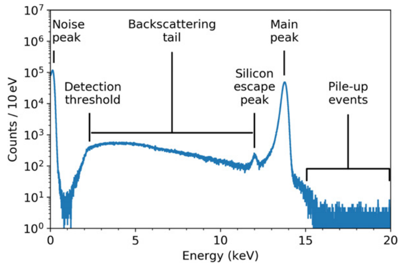
Figure 30: Spectrum of a 14 keV monoenergetic electron beam from an electron microscope measured with a TRISTAN prototype detector. Taken from Ref. [146].
