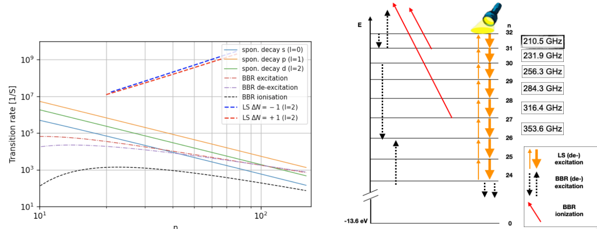
Figure 23: Left: Transition rates for the different processes the Rydberg atoms undergo in the main spectrometer for low angular momenta l . The blackbody-radiation-induced ionization peaks at about n = 25 . Even at a radiance of only 0.005 \text{ W/m}^2 , the transition rate for light-source-induced de-excitation is about 5 orders of magnitude higher than for ionization induced by blackbody radiation. Right: Simplified transitions and binding-energy diagram of hydrogen. The thicker arrow for light-source-induced de-excitation indicates the higher ionization rates for this process compared to the excitation channel (compare with left panel).
