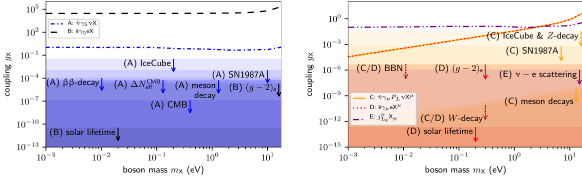
Figure 12: The lines show the statistical sensitivity (90% C.L.) of KATRIN for the detection of eV-scale light pseudoscalars emitted from neutrinos (A) or from electrons (B) (left) and vector bosons emitted from neutrinos (C), from electrons (D), or from both (E) (right). The shaded areas mark the parameter regions allowed from other constraints. Figures taken from Ref. [99].
