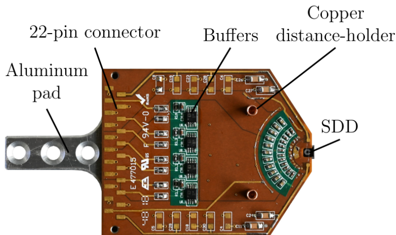
Figure 32: Photograph of the board hosting the TRISTAN FBM detector. Reproduced with permission from Ref. [149].
