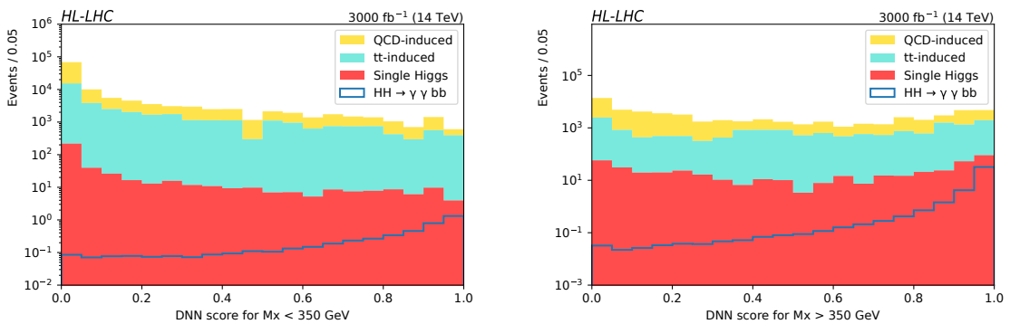
Figure 12: (Left) DNN score for the M_1 < 350 GeV region. (Right) DNN score for the M_1 > 350 GeV region. Histograms are scaled to cross section and luminosity. The background processes are stacked.
