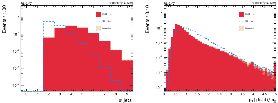
Figure 4: (Left) Number of jets per event and (Right) transverse momentum of the leading jet divided by the invariant mass of the dijet object, for signal and t\bar{t}H background. Histograms are scaled to unity to compare the shapes.
