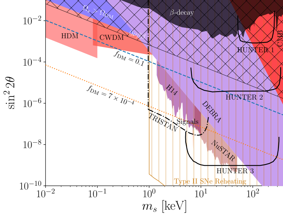
Figure 6. The parameter space of interest for low-reheating temperature Universes and keV-scale neutrinos is shown ( T \approx 5 MeV). This is an update to the limits from [260], with the X-ray limits reflecting production at the given mass and mixing angle parameter space, with projected limits from the HUNTER experiment’s proposed phases [299], and from KATRIN/TRISTAN [286]. The diagonally hatched region refers to the double beta decay limit mentioned in the text. The red region in upper right is from CMB distortion limits. The purple region is from diffuse x-ray background observations.
