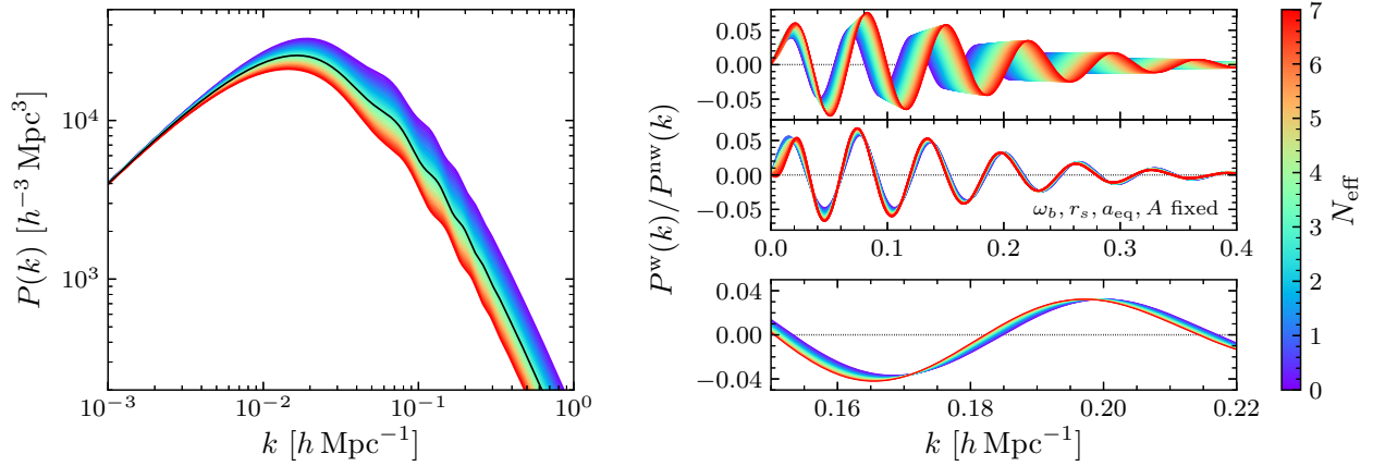
Figure 4. Variation of the matter power spectrum P(k) (left) and the BAO spectrum P^w(k)/P^{nw}(k) (right) as a function of N_{\text{eff}} (adapted from [86]). The BAO spectrum is the ratio of the oscillatory part P^w(k) of the matter power spectrum and its smooth broadband part P^{nw}(k) = P(k) - P^w(k) . The physical baryon density, \omega_b , the physical sound horizon at the drag epoch, r_s , the scale factor at matter-radiation equality, a_{\text{eq}} , and the BAO amplitude A at the fourth peak are held fixed in the second BAO panel. This panel and the bottom zoom-in show the remaining phase shift induced by free-streaming relativistic species. We refer to [86] for additional details.
