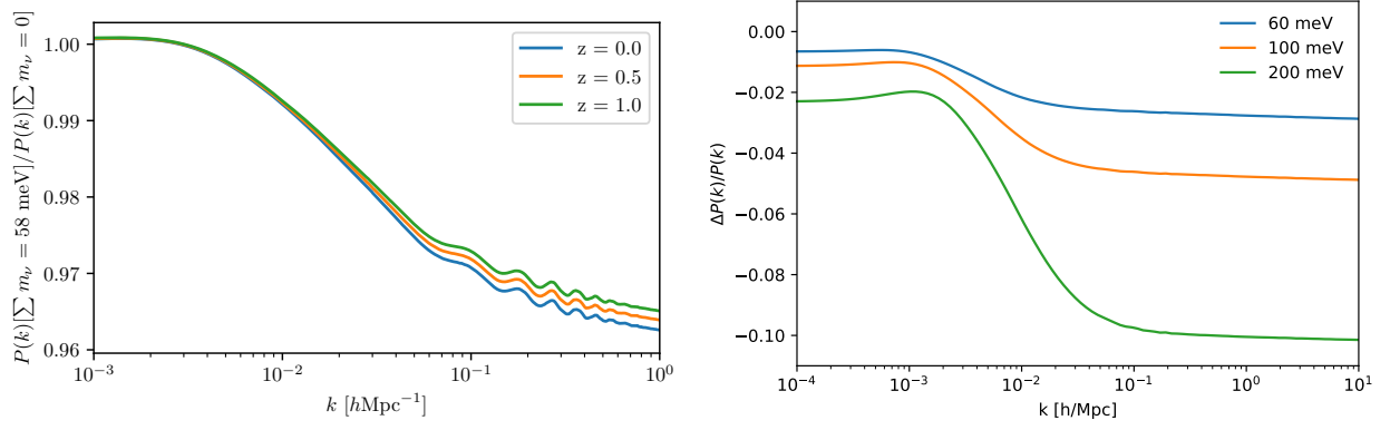
Figure 2. Left: Suppression of the matter power spectrum due to massive neutrinos at selected redshifts computed with CLASS [102]. The comparison is made at fixed H_0 , \Omega_m h^2 , \Omega_b h^2 , and A_s . Right: Relative suppression effect on the power spectrum at z = 0 caused by neutrinos with varying total mass \sum m_\nu , with parameters \Omega_c , \Omega_b and H_0 kept constant. Large-scale structure experiments have little sensitivity at scales k < 10^{-2} h/\text{Mpc} and can mostly resolve the suppressed part of the spectrum.
