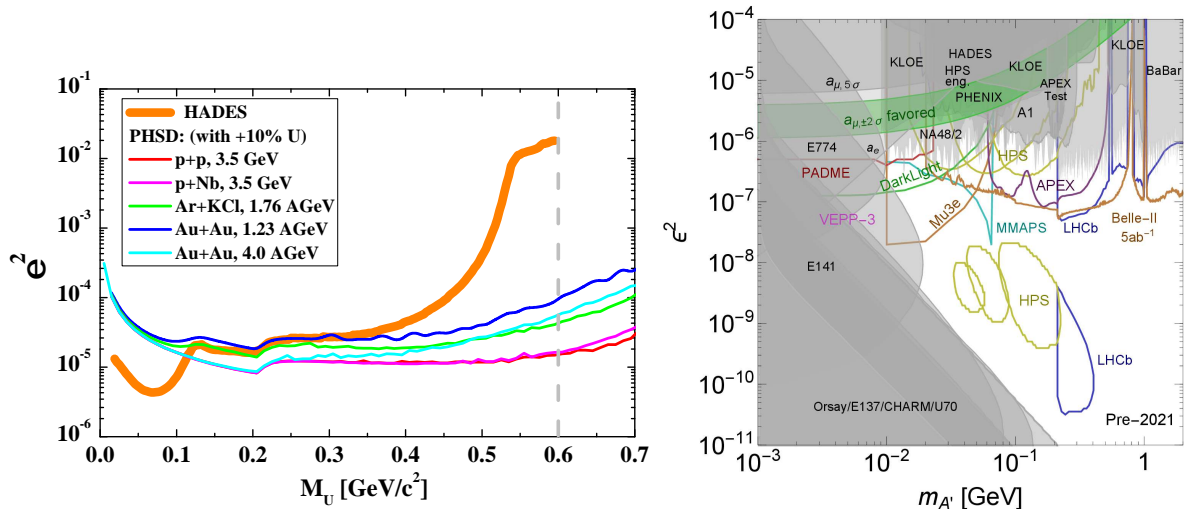
Figure 4: Left: Kinetic mixing parameter \epsilon^2 extracted from the PHSD dilepton spectra for p-p at 3.5 GeV (red line), p-Nb at 3.5 GeV (magenta line), Ar-KCl at 1.76 AGeV (green line), Au-Au at 1.23 AGeV (blue line), Au-Au at 4.0 AGeV in comparison with the combined HADES results (orange line) [101]. The PHSD results are shown with 10% allowed surplus of the U -boson contributions over the total SM yield, i.e. C_U = 0.1 . Right: Compilation of the experimental upper limits for \epsilon^2 versus the mass of dark photon set by worldwide experiments. The figure is taken from Ref. [100].
