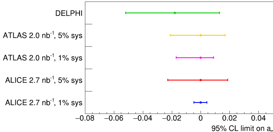
Figure 2: Expected 95% C.L. limits on a_\tau measurements with available ATLAS/CMS Run 2 data ( 2\text{ nb}^{-1} ) and with future ALICE data to be collected in 2022 ( 2.7\text{ nb}^{-1} ) for two different assumptions on systematic uncertainty (1%, 5%) in comparison with DELPHI results [23].
