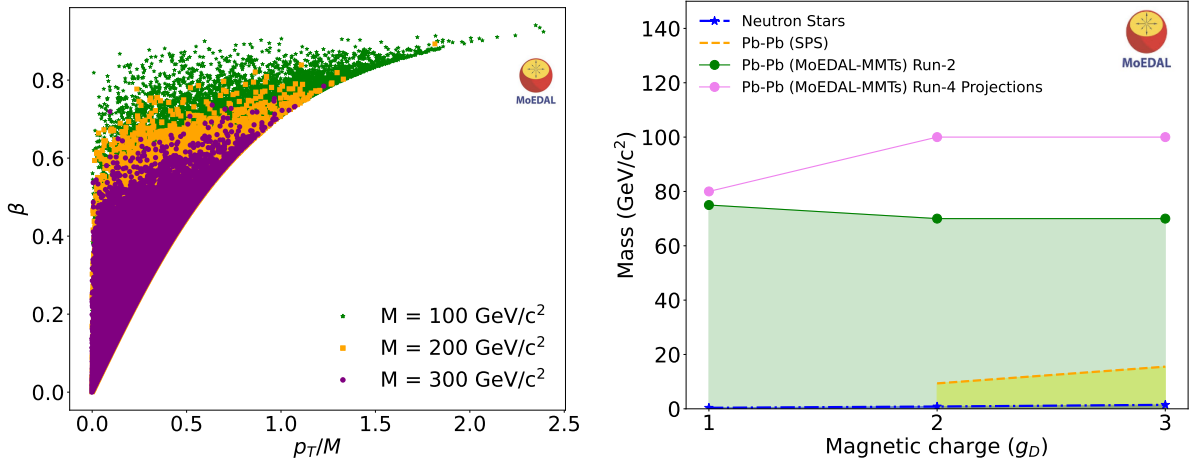
Figure 3: Left: Transverse momentum distribution for Schwinger MMs derived from the free-particle approximation, as a function of MM mass ( M ) plotted versus MM velocity \beta . Right: The 95% C.L. mass exclusion regions obtained from MoEDAL’s search in Pb-Pb collisions at the LHC [43]. The conservative exclusion region is shaded in green. The projected limits for future Pb-Pb runs using the conservative Schwinger cross section and the MoEDAL-MMTs are also shown.
