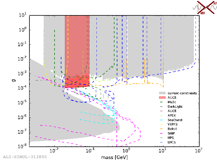
Figure 5: Dark photon limits in the coupling vs. mass plane. The red area indicates the expected 90% C.L. constraints from ALICE measurements before 2030. Figure adapted from Ref. [2].
