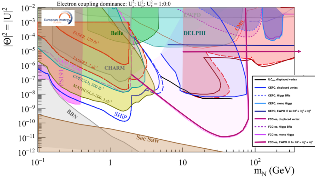
Figure 8: Expected sensitivity to Heavy-Neutral Leptons (a.k.a. Right Handed Neutrinos) in various future facilities. The reach of FCC-ee is for very small heavy-light mixing angle in Z decays, down to the see-saw limit; it is complemented up to very high masses (60 TeV or more) for heavy-light neutrino mixing larger than 10^{-5} by constraints from Electroweak and tau decay precision measurements. See [1], Fig 8.19.
