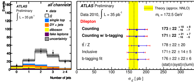
Figure 1: Jet multiplicity distribution without the N_{jets} \leq 2 and b -tagging requirements(left). The \sigma_{t\bar{t}} cross section measurements from different methods(right).
