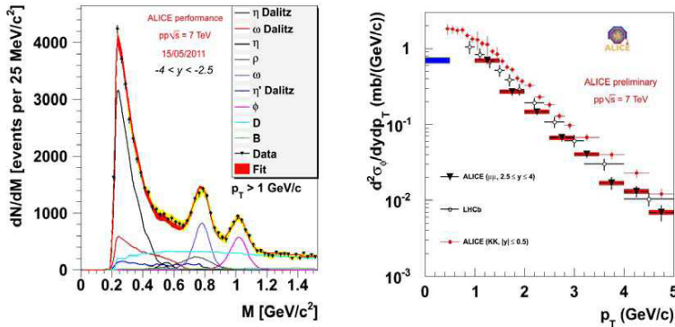
(a) Dimuon mass spectrum for p_T > 1 \text{ GeV}/c . (b) Differential cross section d^2\sigma_{\phi}^2/dydp_T as a function of p_T .
