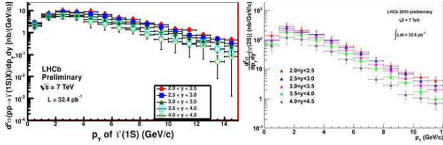
Figure 2: \Upsilon(1S) (left) and \psi(2S) (right) cross section in the dimuon mode.
