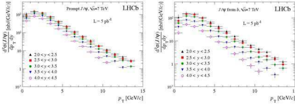
Figure 1: J/\psi cross section for prompt (left) and delayed (right) component.
